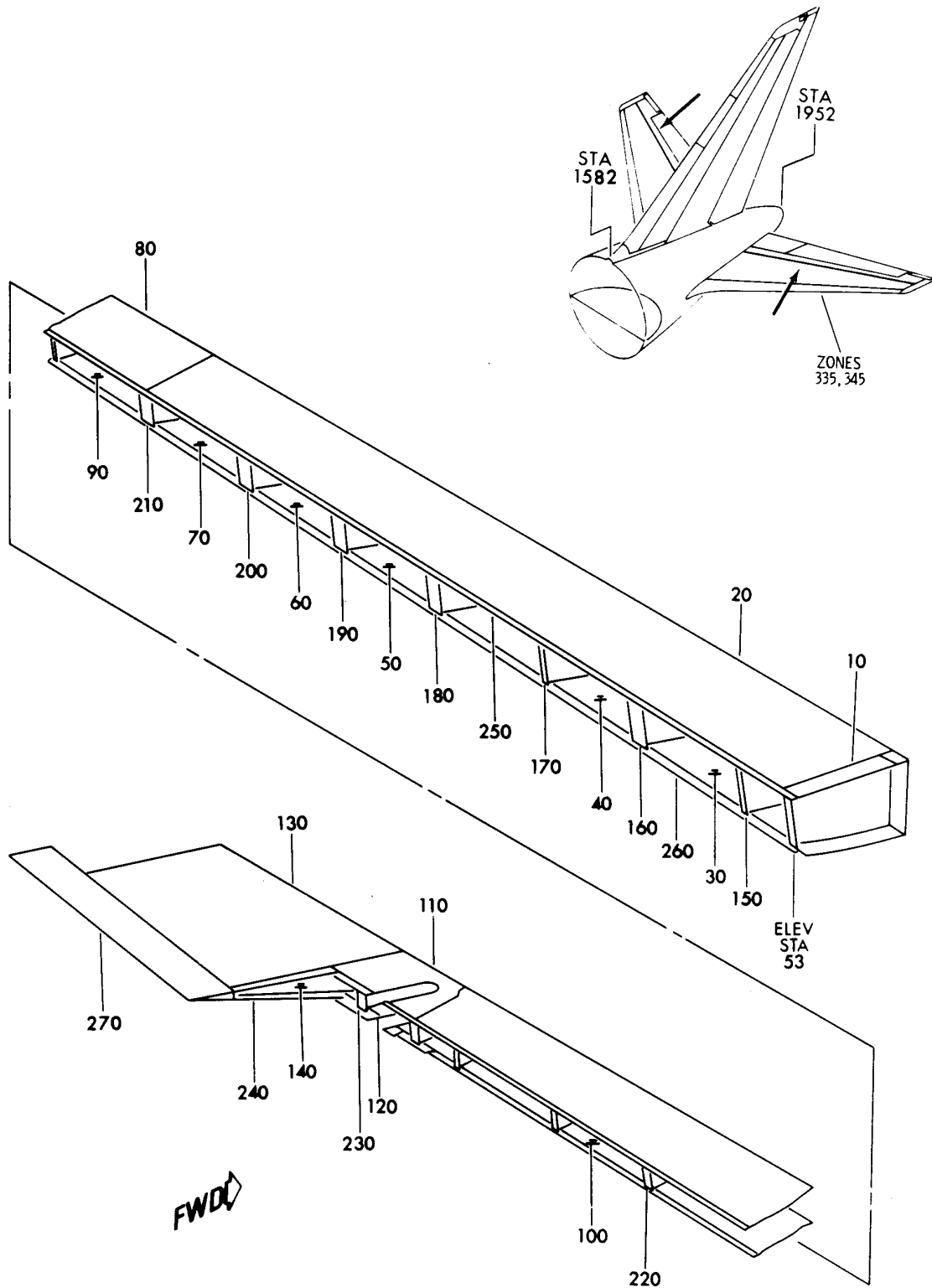
TRAILING EDGE INSTL-FXD HORIZ STAB. FIGURE 1
