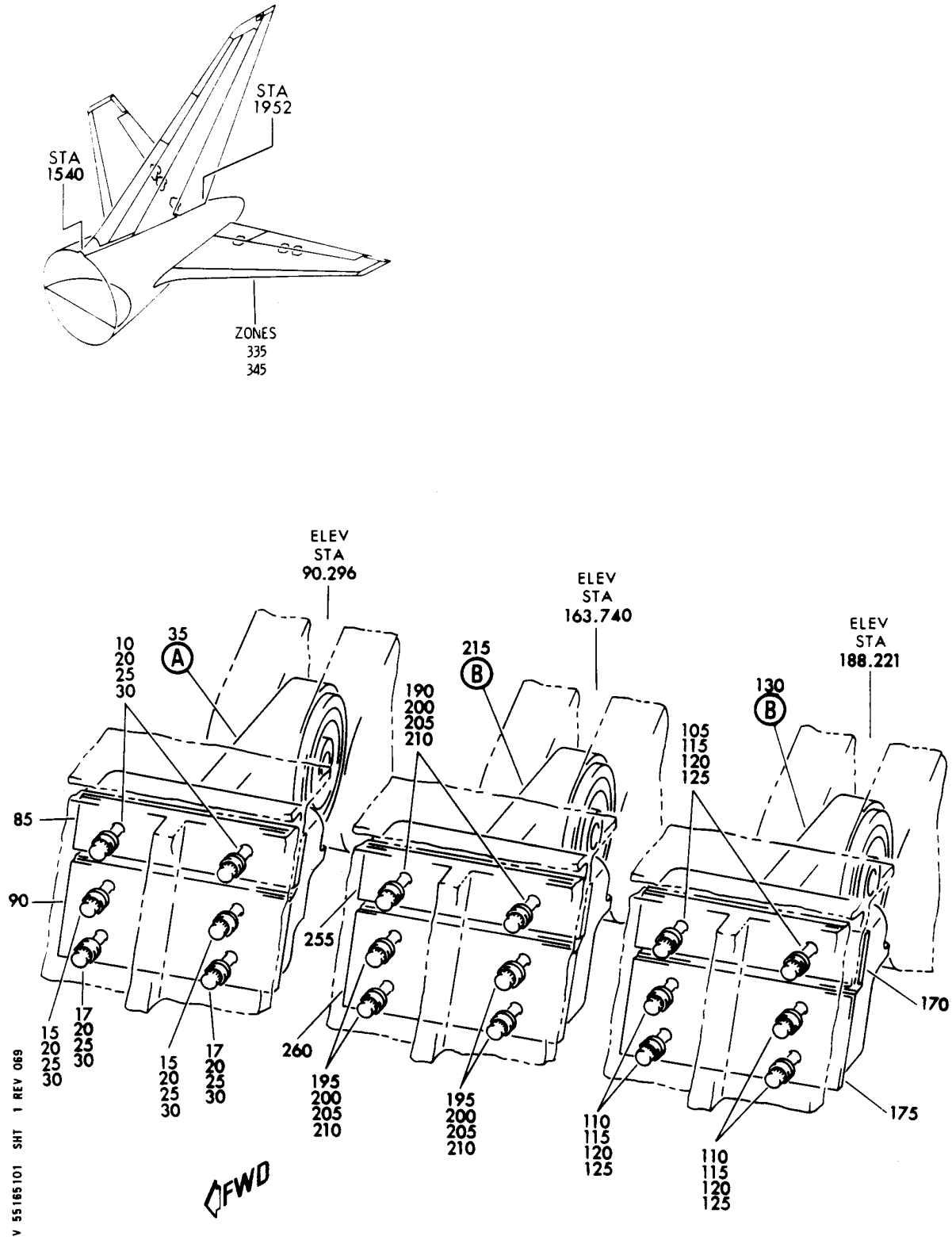
RIB INSTL-HORIZ STAB. FXD T E FIGURE 1 (SHEET 1)
