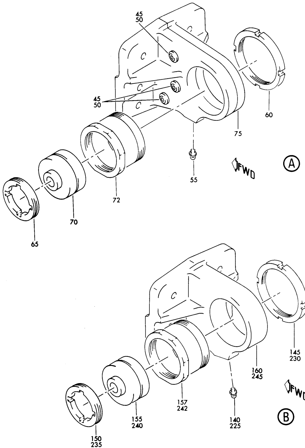
RIB INSTL-HORIZ STAB. FXD T E FIGURE 1 (SHEET 2)
