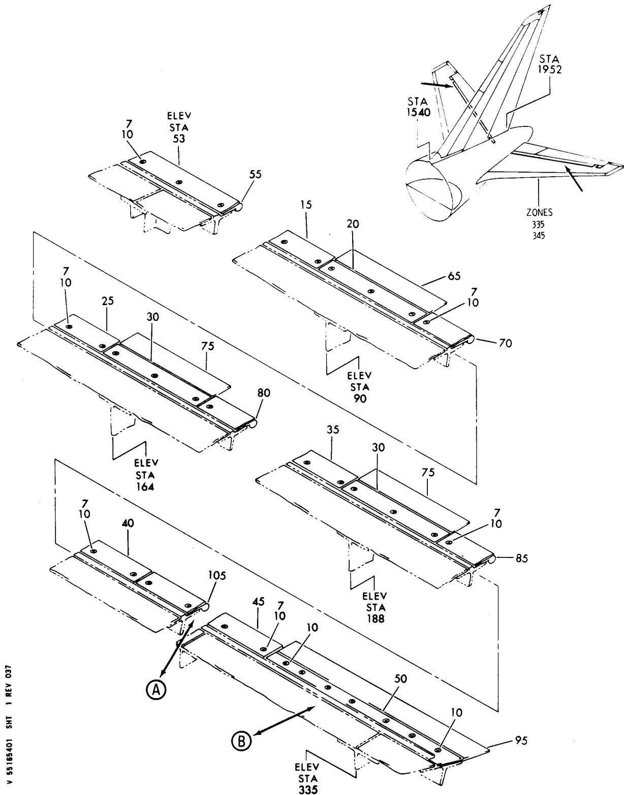
BEAM INSTL-HORIZ. STAB. FXD TE UPR FIGURE 1 (SHEET 1)
