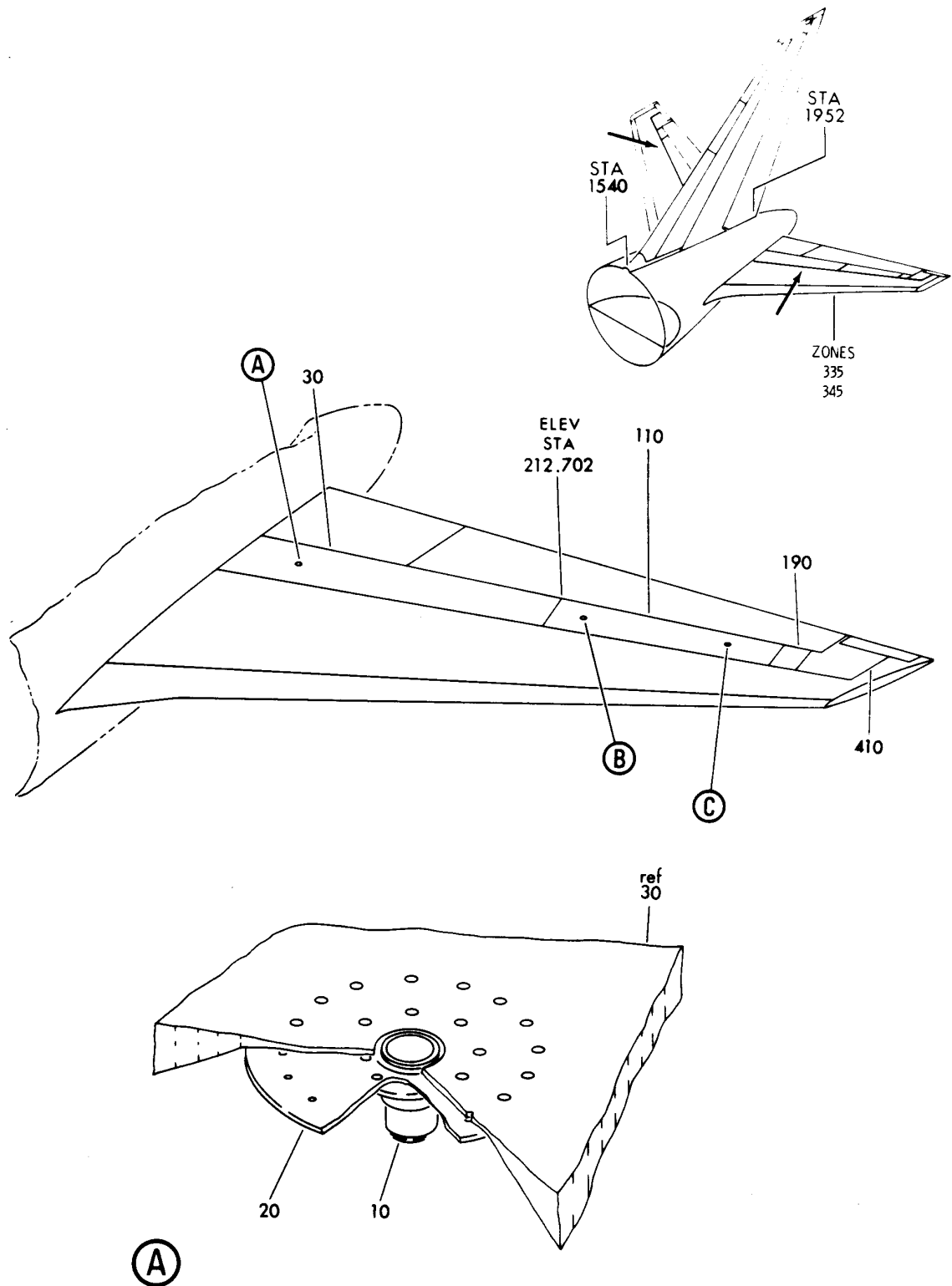
PANEL INSTL-HORIZ STAB. ELEV FXD TE UPR FIGURE 1 (SHEET 1)
