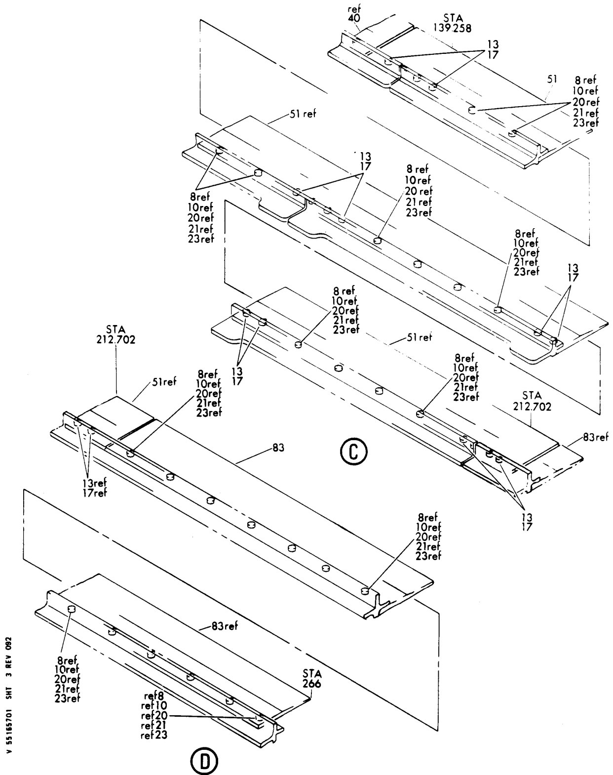
BEAM INSTL-FXD TE HORIZ STAB. LWR FIGURE 1 (SHEET 3)
