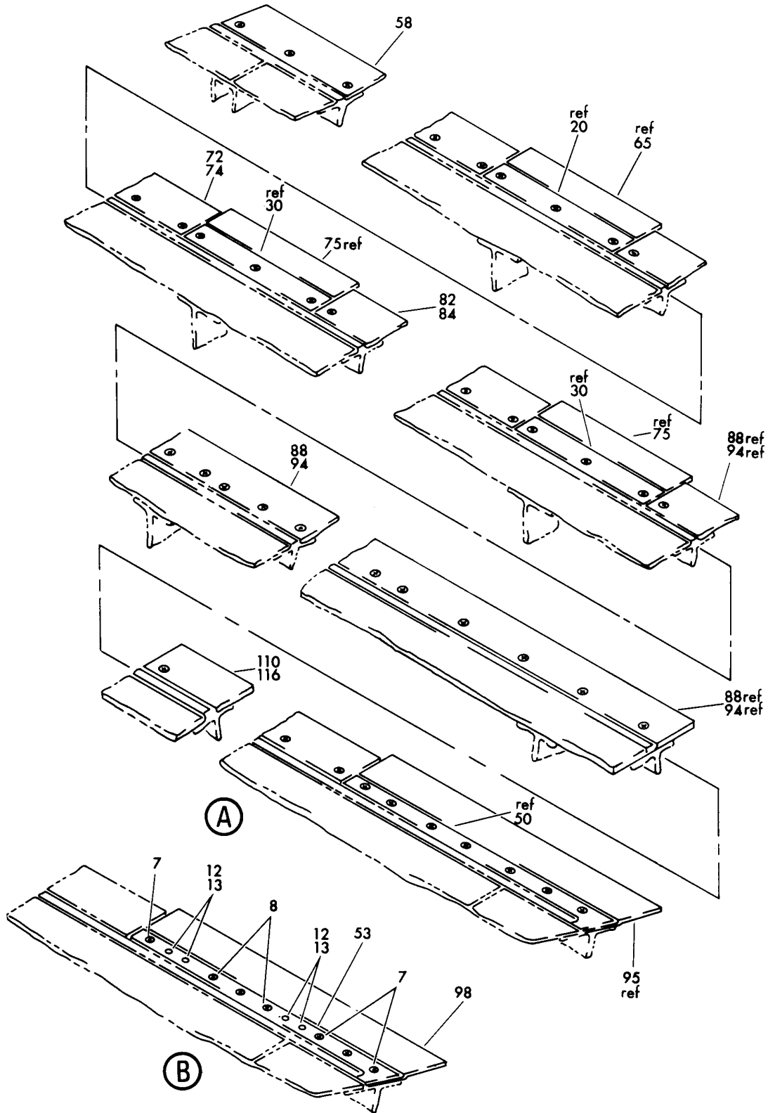
BEAM INSTL-HORIZ. STAB. FXD TE UPR FIGURE 1 (SHEET 2)
