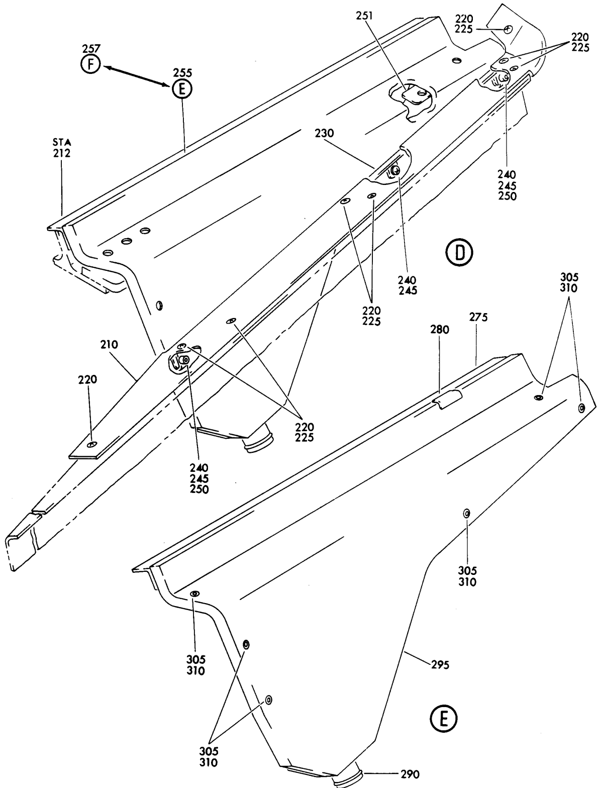
LINING INSTL-SILL NO. 2 AND NO. 3 WINDOW LWR FIGURE 1 (SHEET 2)
