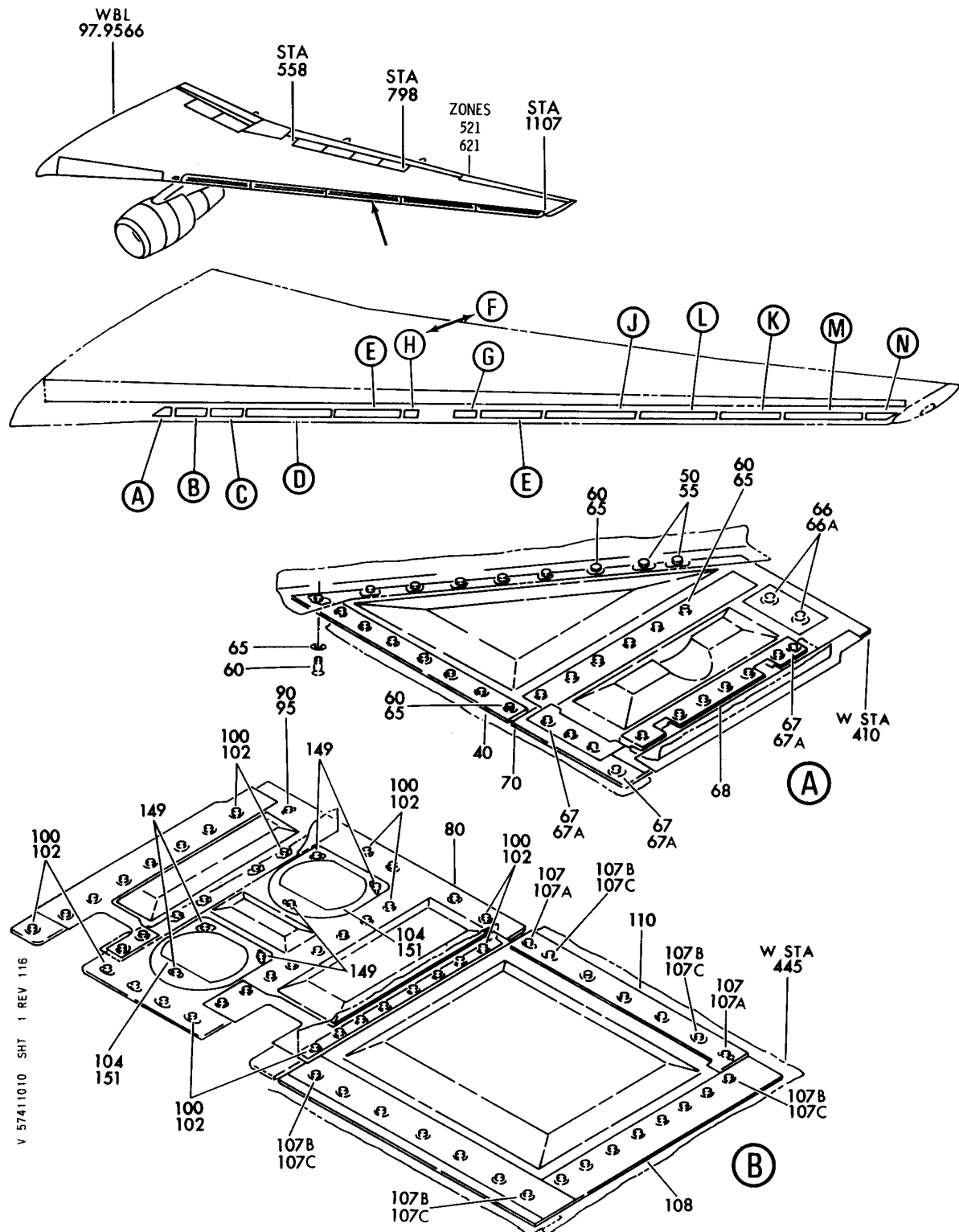
PANEL INSTL-FXD LE OUTBD WING LWR FIGURE 10 (SHEET 1)
