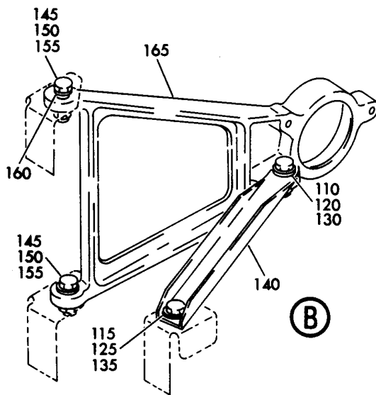
SUPPORT INSTL-BODY LE SLAT DRIVE BRG FIGURE 1
