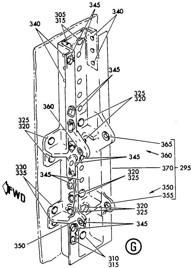
BEAM INSTL-WS 308 TO WS 375 SPOILER FIGURE 1 (SHEET 5)
