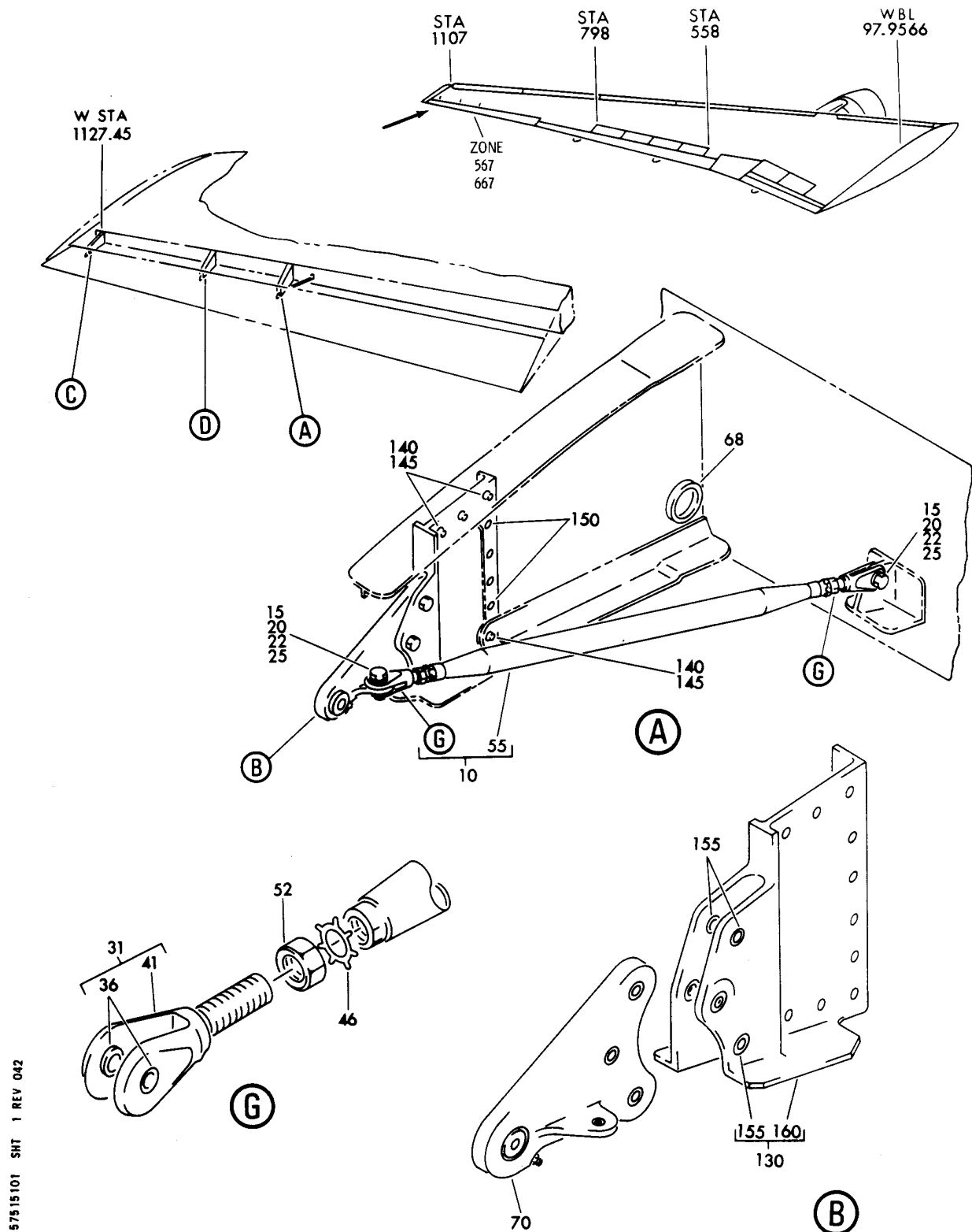
RIB INSTL-PREMODULE AIL. HINGE SPRT FIGURE 1 (SHEET 1)
