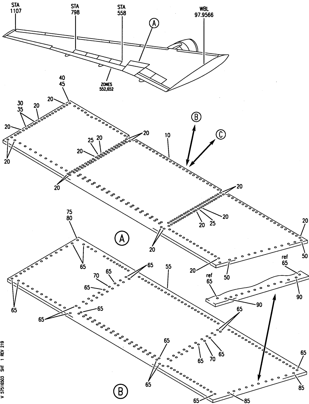
PANEL INSTL-OUTBD UPR WING FXD TE FIGURE 3 (SHEET 1)
