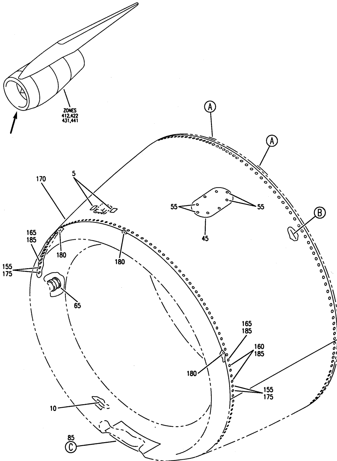
INLET ASSY-PW4000 ENG (INLET COWL ONLY) FIGURE 10A (SHEET 1)
