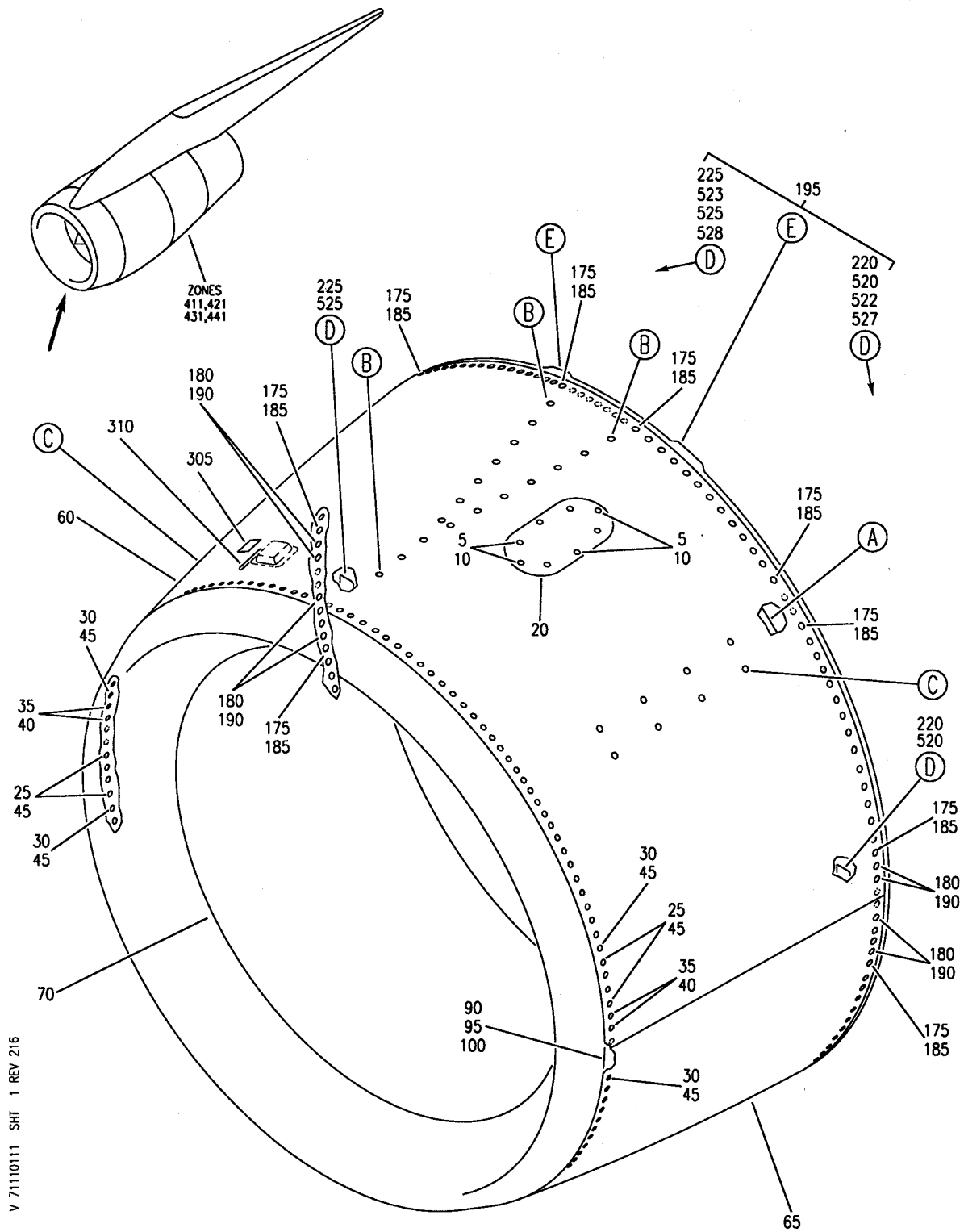
INLET ASSY-PW4000 ENG FIGURE 11 (SHEET 1)
