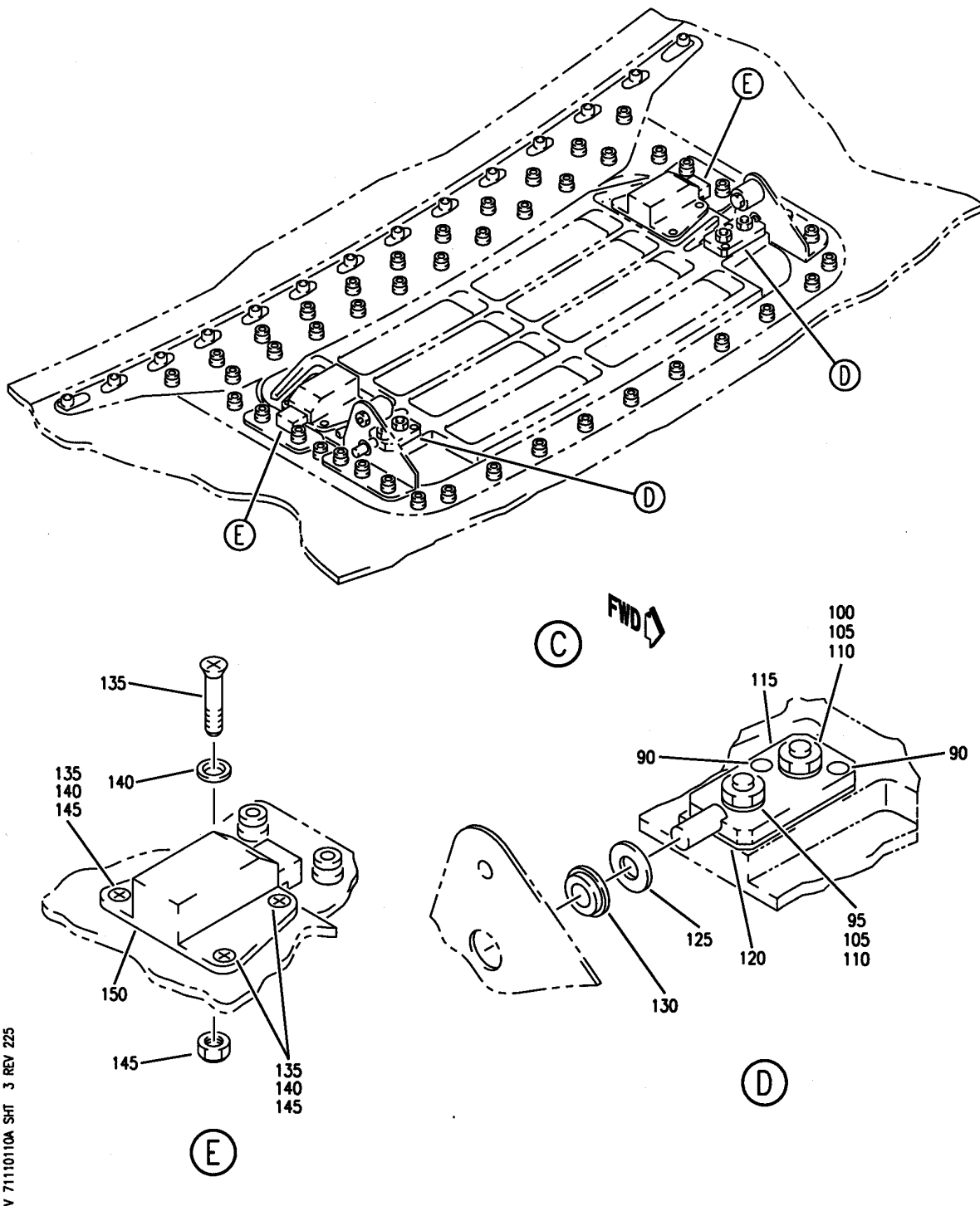
INLET ASSY-PW4000 ENG (INLET COWL ONLY) FIGURE 10A (SHEET 3)
