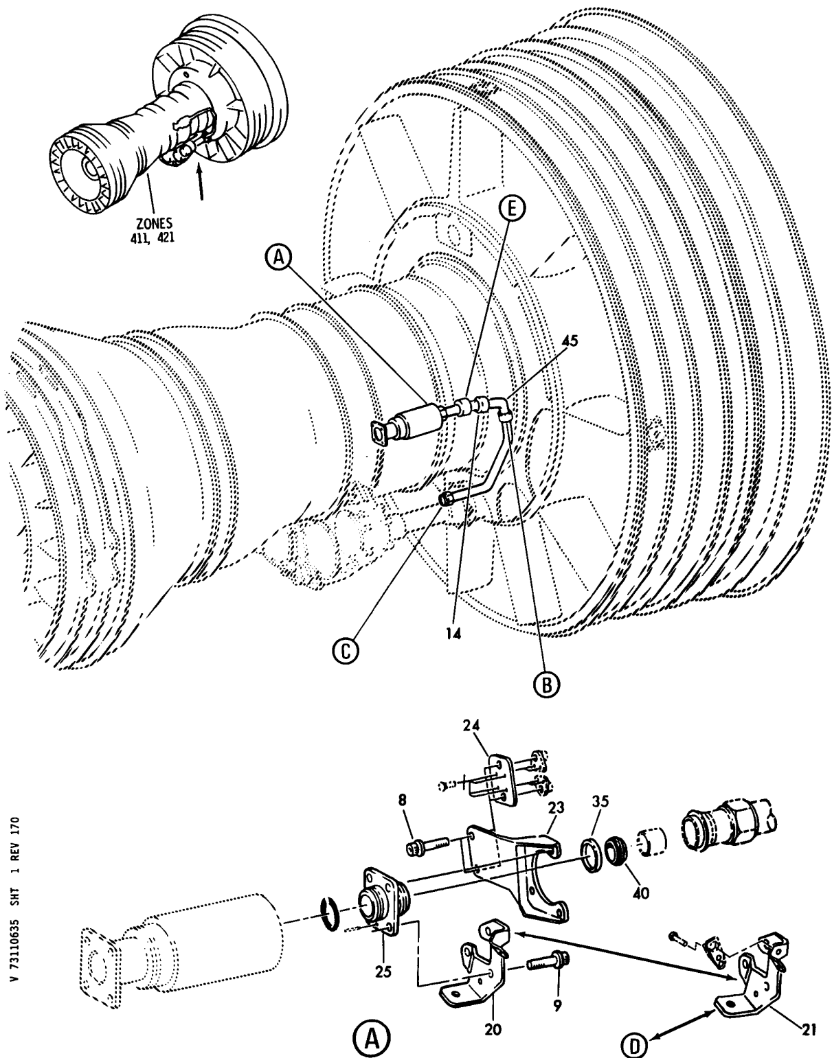
TUBE-FUEL DISTR VALVE SUPPLY (PW4000) FIGURE 35 (SHEET 1)
