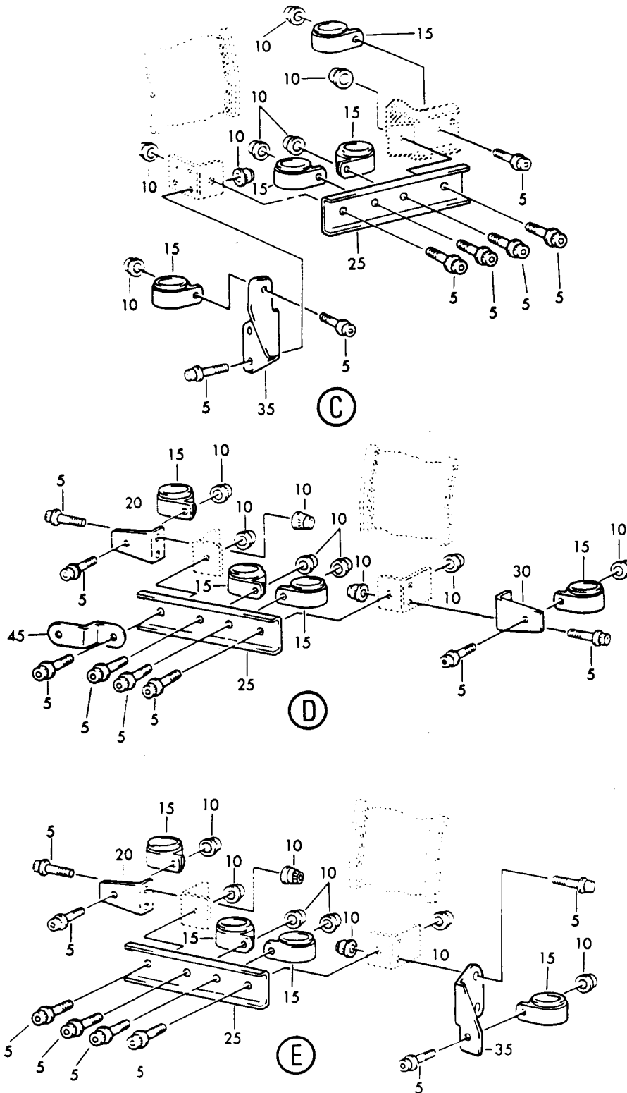
BRACKETS AND SUPPORT-HIGH PRESSURE TURB CASE COOLING (PW4000) FIGURE 5 (SHEET 2)
