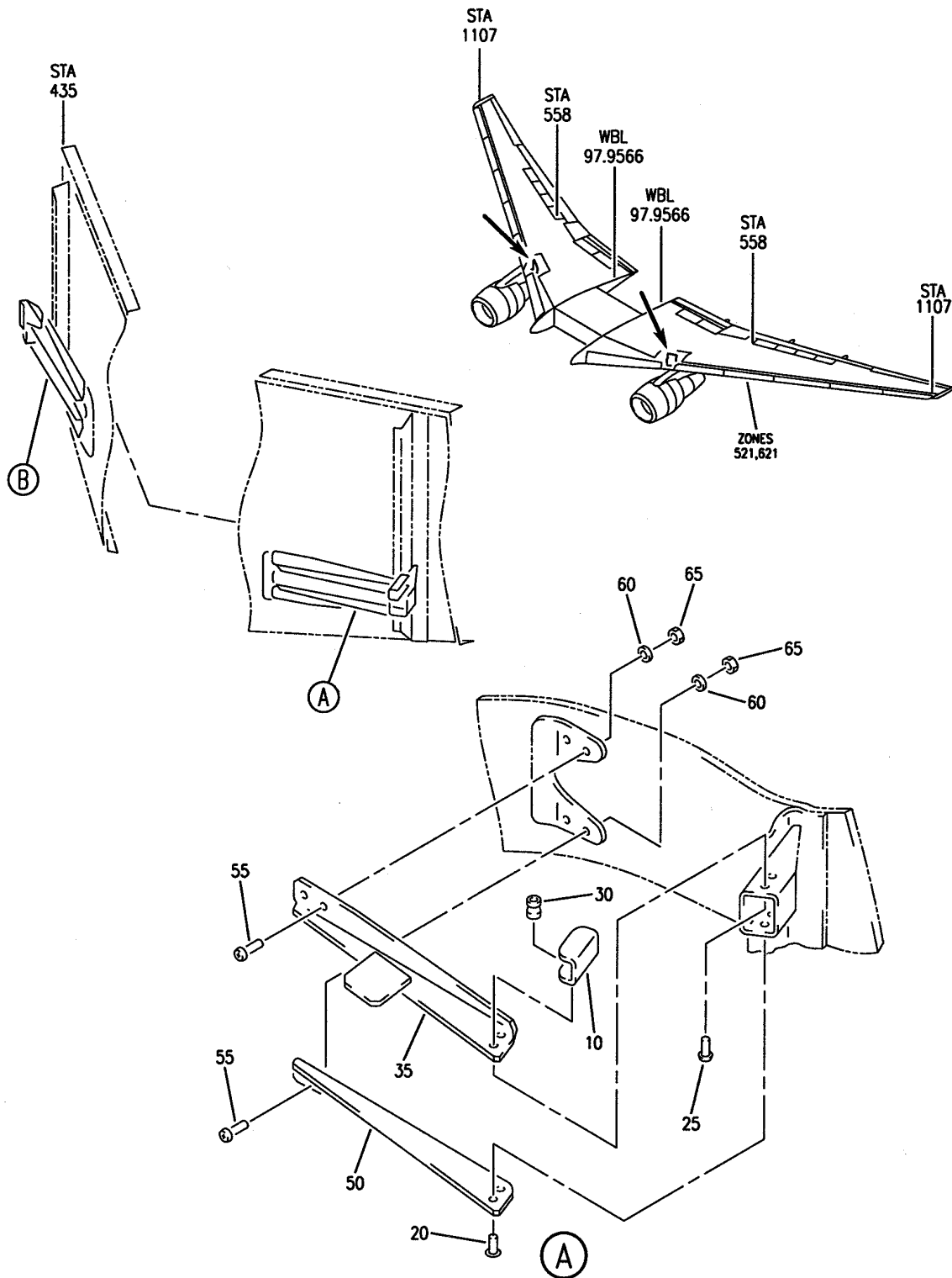
BRACKET INSTL-STOP ENG THRUST CONT CABLE WING OFS STA 368.21 FIGURE 2 (SHEET 1)
