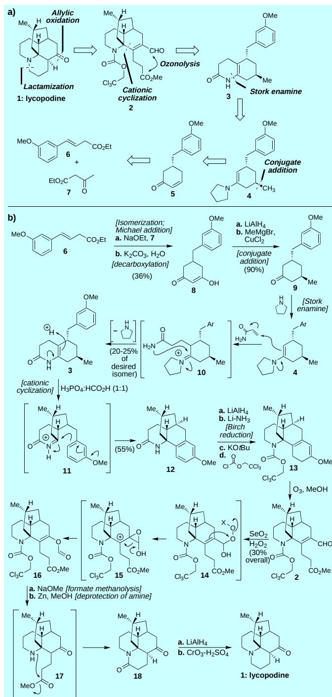
Scheme 9. a) Strategic bond disconnections and retrosynthetic analysis of (±)-lycophodine and b) total synthesis (G. Stork et al., 1968). [72]
