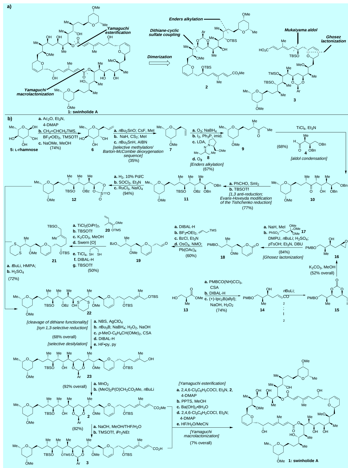
Scheme 32. a) Strategic bond disconnections and retrosynthetic analysis of swinholide A and b) total synthesis (Nicolaou et al., 1995). [171]
