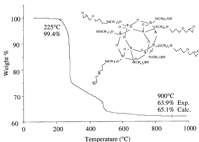
Figure 3 TGA of (glycidyl) 4 (HD) 4 T 8 cube. Average substitution \approx 4 .
