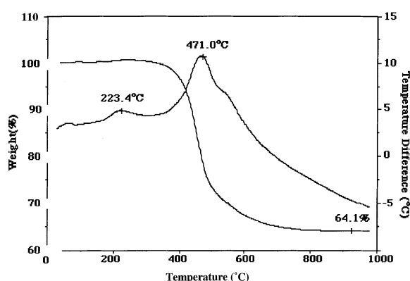
Figure 4 TGA/DTA of tetra-allylcyclohexenyl-substituted cube heated at 10 °C min -1 in air.
