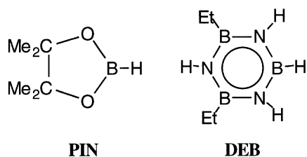
Figure 7 Monofunctional boranes: pinacolborane (PIN), and B -diethylborazine (DEB).
