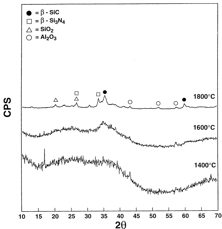
Figure 9 Powder XRD spectra of PIN-HPZ-3 pyrolyzed to (a) 1400 °C, (b) 1600 °C and (c) 1800 °C. (The \text{Al}_2\text{O}_3 impurity comes from the pestle and mortar used to grind the sample.)
