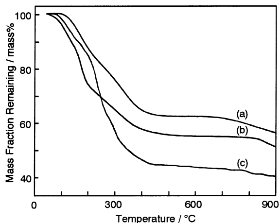
Figure 2 TG curves of the reaction products of \text{Ti}(\text{NMe}_2)_4 with (a) \text{H}_2\text{NCH}_2\text{CH}_2\text{NH}_2 (PreH), (b) \text{HN}(\text{CH}_2\text{CH}_2)_2\text{NH} (PreP) and (c) \text{Me}(\text{H})\text{NCH}_2\text{CH}_2\text{N}(\text{H})\text{Me} (PreMe) under He at a heating rate of 10\text{ }^\circ\text{C min}^{-1} .
