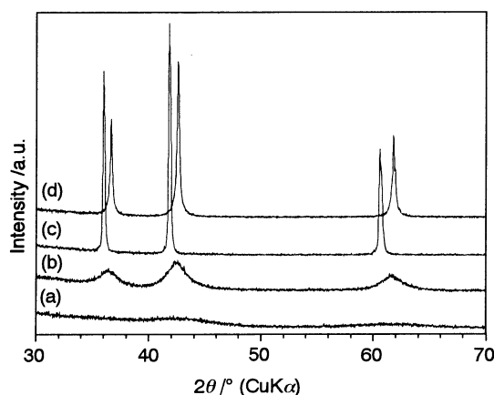
Figure 3 XRD patterns of the reaction product of Ti(NMe 2 ) 4 with H 2 NCH 2 CH 2 NH 2 (PreH) pyrolyzed under argon at (a) 600 °C, (b) 1000 °C, (c) 1500 °C; and (d) pyrolyzed under NH 3 -N 2 (for conditions see the Experimental section).
