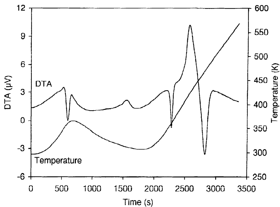
Figure 6 Thermogram of \text{Cp}_2\text{VMe}_2 showing the reversibility of the DTA melting peak (left) and the temperature program (right). He carrier gas ( 1 \text{ l h}^{-1} ).
