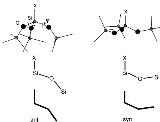
Figure 6 Anti ( \varphi = 0^\circ ) and syn ( \varphi = 180^\circ ) conformations of XSi(OSiMe 3 ) 3 .
