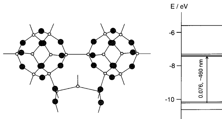
Figure 11 Structure and energy levels of (H_6Si_8O_{12})_2(Si(OH)_2)_2SiH_2 . This substance exhibits an oscillator strength of 0.076 for the strongest transition at ca 460 nm.
