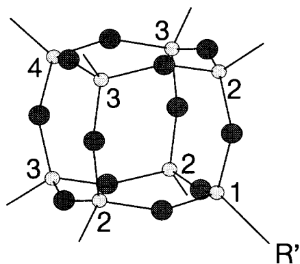
Figure 3 The four sets of equivalent silicon atoms in monosubstituted silasesquioxanes.
