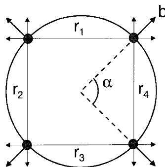
Figure 9 Idealized ring-opening coordinates for the general case of N atoms equally spaced on a ring (left-hand side), and for the four-membered-ring (right-hand side).
