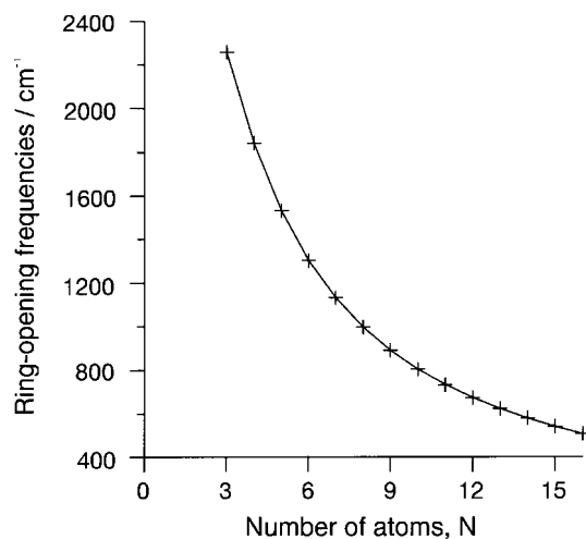
Figure 10 Totally symmetric ring-opening frequencies for rings of different sizes: N = 3-16 ; f = 1 \text{ mdyn } \text{Å}^{-1} ; m = 1 \text{ u} .
