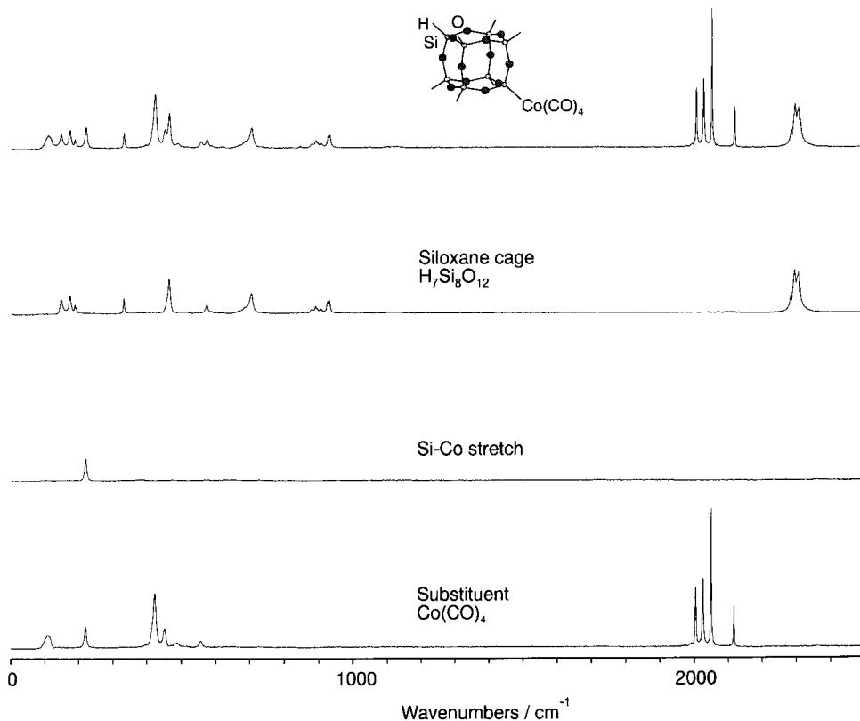
Figure 5 Fourier-transform Raman spectrum of [\text{Co}(\text{CO})_4(\text{H}_7\text{Si}_8\text{O}_{12})] divided into the lines due to the siloxane cage, the substituent and the Si-Co stretch.
