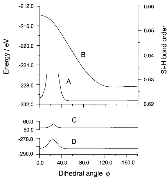
Figure 7 Energies and bond order of HSi(OSiMe 3 ) 3 as a function of the dihedral angle \varphi (A): total energy E_{\text{tot}} ; (B) Si–H bond order; (C) core–core repulsion E_{\text{rep}} ; (D) extended-Hückel binding energy ( \Delta E_{\text{EHMO}} ). The barrier in the total energy (A) at about 30^\circ is enormous and caused by orbital interactions (D) and core–core repulsion (C).
