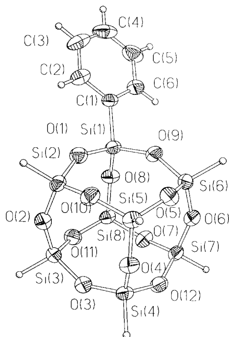
Figure 2 Crystal structure of PhH_7Si_8O_{12} with atomic labeling and anisotropic displacement parameters at the 30% probability level.
