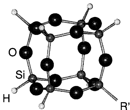
Figure 1 The octasilasesquioxane cage R'R_7Si_8O_{12} for R = H .
