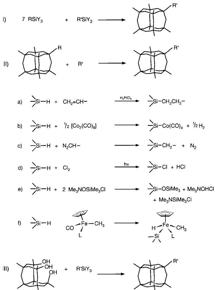
Scheme 1 Three general ways (I–III) of synthesizing monosubstituted octasilasesquioxanes.
