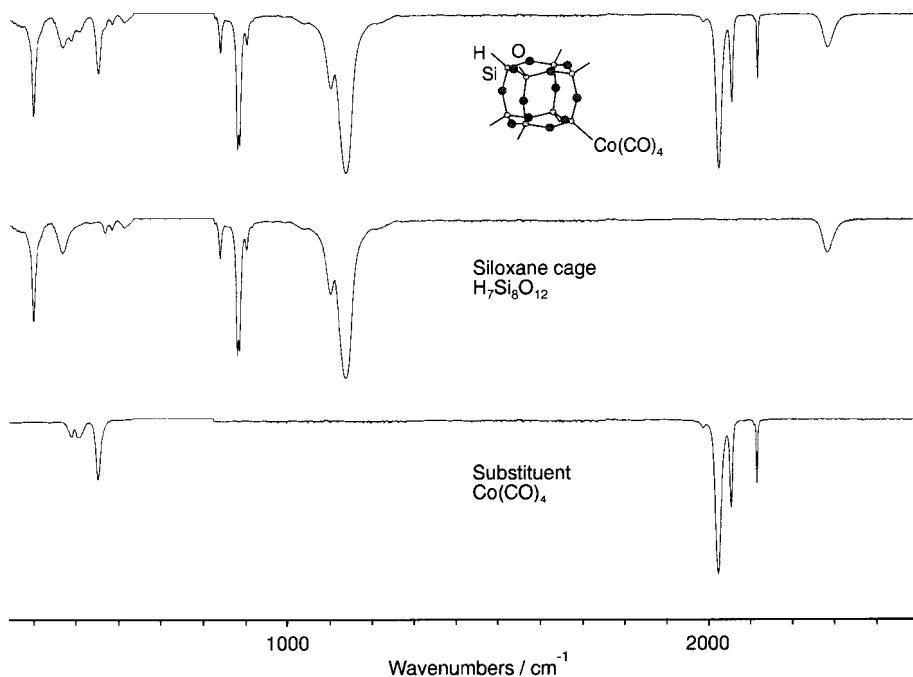
Figure 4 Transmission IR spectrum of [\text{Co}(\text{CO})_4(\text{H}_7\text{Si}_8\text{O}_{12})] divided into the lines due to the siloxane cage and the substituent.
