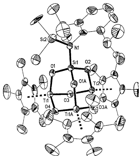
Figure 3 A perspective view of the molecular structure of 16 .
