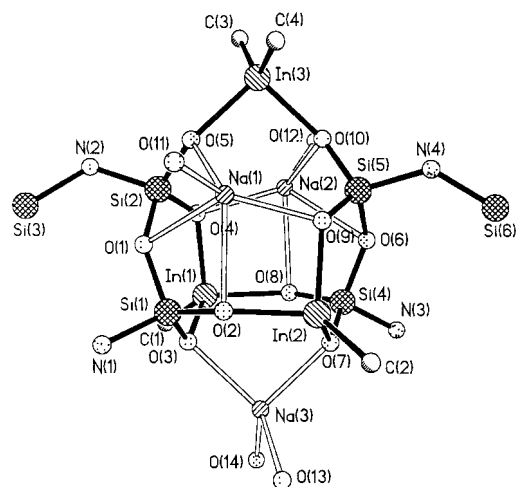
Figure 9 Molecular structure of the In–Na–O–Si core of 44 .
