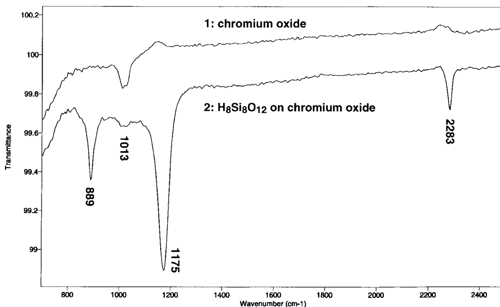
Figure 3 RAIRS spectrum of a thin chromium oxide film on chromium (spectrum 1), and H 8 Si 8 O 12 absorbed on chromium oxide (2).
