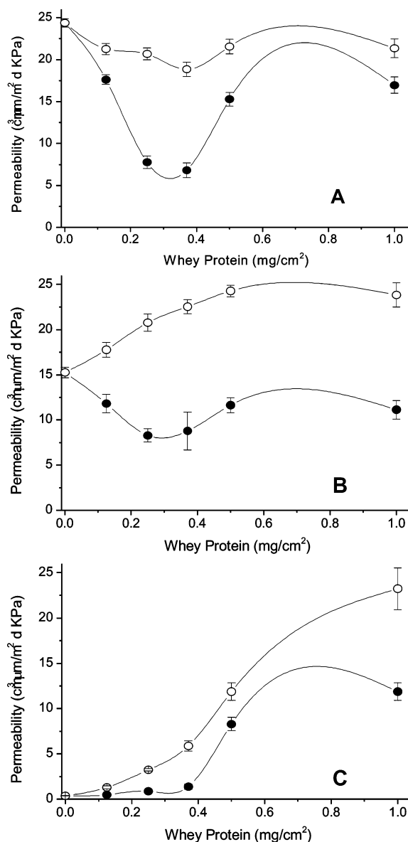
Figure 5. Influence of protein concentration on the permeability to oxygen (A), carbon dioxide (B), and water vapor (C) of CWP films prepared in the absence (○) and presence (●) of TGase.
