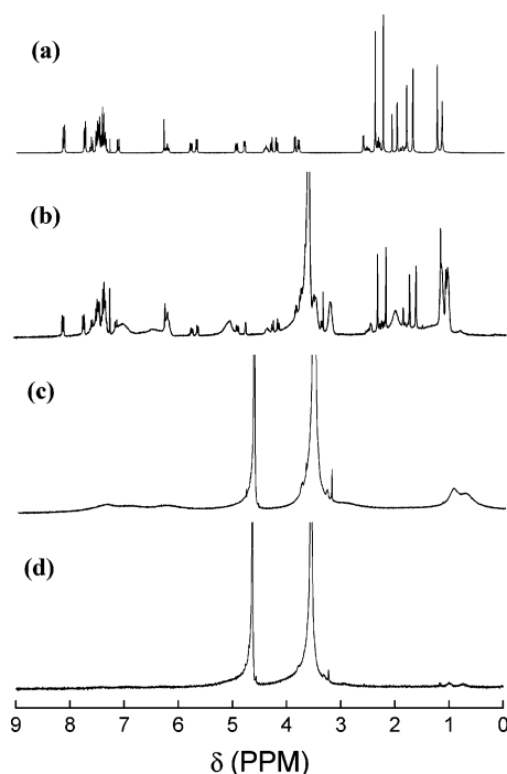
Figure 4. 1 H NMR spectra of paclitaxel in CDCl 3 (a), paclitaxel-loaded micelles in CDCl 3 (b), micelles without paclitaxel in D 2 O (c), and paclitaxel-loaded micelles in D 2 O (d).
