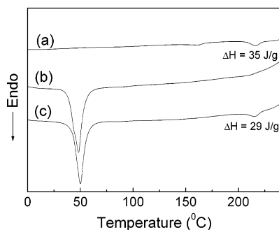
Figure 6. DSC thermograms of paclitaxel (a), 31.7 wt % paclitaxel-loaded micelles (b), and a mixture of paclitaxel and micelles (c). The amount of paclitaxel in each sample was the same for all samples.
