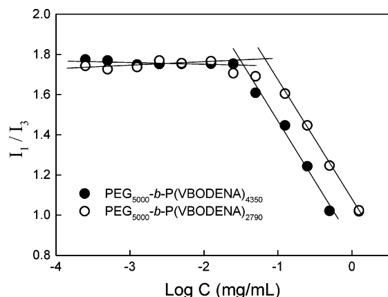
Figure 2. Intensity ratios ( I_1/I_3 ) of pyrene emission spectra as a function of the concentrations of PEG 5000 - b -P(VBODENA) 4350 and PEG 5000 - b -P(VBODENA) 2790 .
