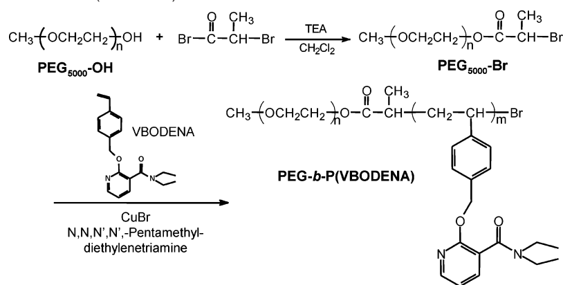
Scheme 1. Synthetic Route for PEG- b -P(VBODENA)
