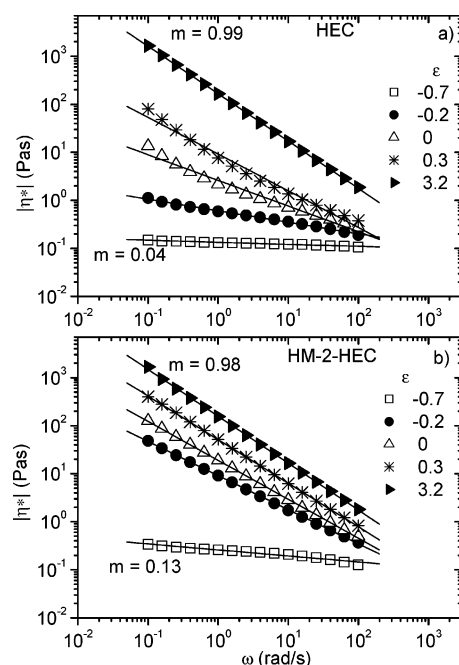
Figure 8. Frequency dependence of the complex viscosity (log–log plot) at different stages during the gelation process for 2 wt % samples of HEC and HM-2-HEC in the presence of 10 wt % cross-linker agent.
