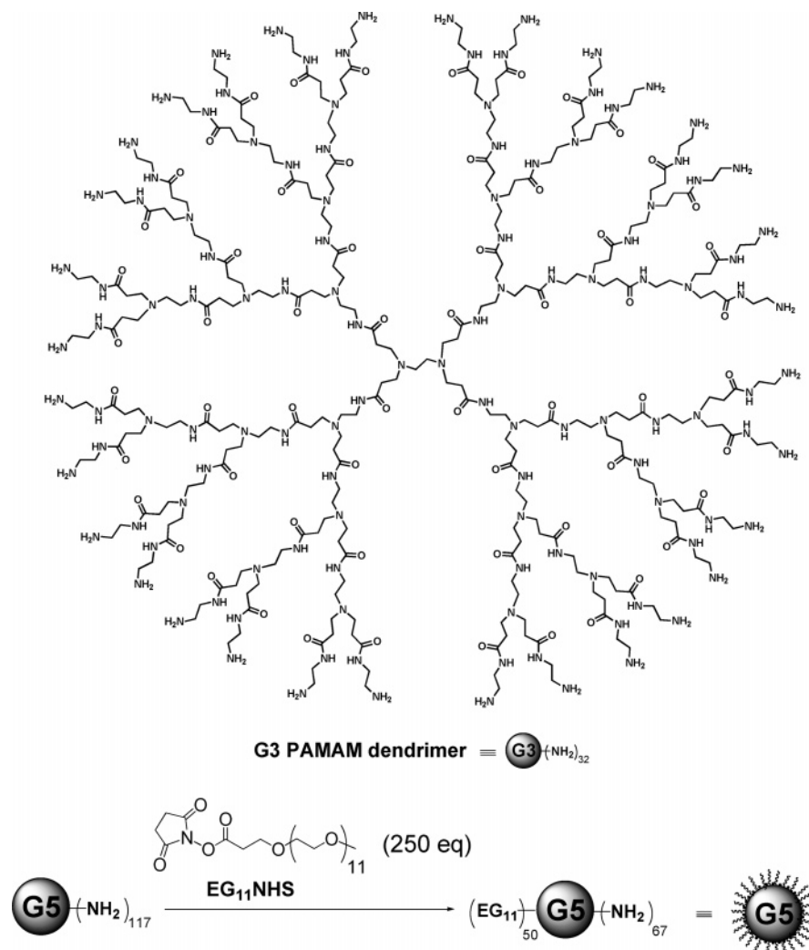
Figure 1. Structure of the G3 PAMAM dendrimer possessing ~32 amino groups at the periphery, and the reaction used in the present study for modifying the commercial G5 PAMAM dendrimer, possessing ~117 amino groups at its periphery, with PEG consisting of 11 ethylene glycol units (EG 11 ).
