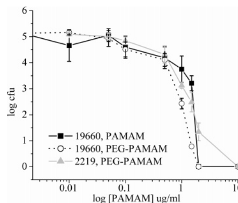
Figure 3. Concentration (cfu/mL) of PA, including PA19660 (lab strain) and PA2219 (clinical strain), upon incubation with PAMAM and PEG-PAMAM at various concentrations for 2 h. The data points are the mean of at least three separate experiments, and the error bar represents the standard deviation.
