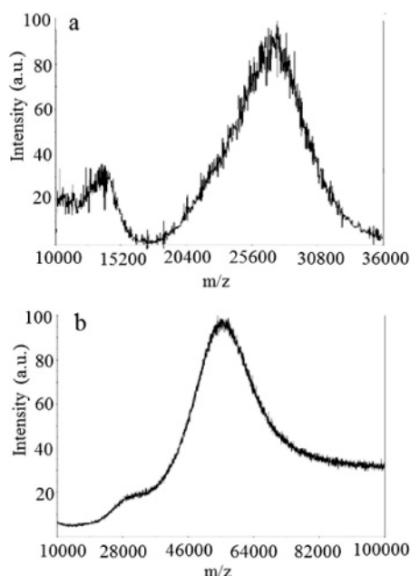
Figure 2. MALDI-TOF mass spectra of the G5 PAMAM (a) and PEG-PAMAM (b), showing their average MWs to be 26 575 and 55 249 Da. The peak at \sim 13\,290 (a) and the shoulder at \sim 27\,600 Da/charge (b) are likely from the double-charged molecular ions.
