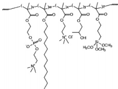
Figure 7. Molecular structure of synthetic cationic phosphorylcholine (PC)-based copolymers used for stent-based release coatings. Reprinted from ref 147. Copyright 2006 American Chemical Society.
