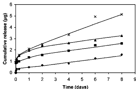
Figure 8. Controlled release of antisense S-ODN from different PC copolymer films (choline methacrylate monomer content: 0%, \diamond ; 5%, \blacksquare ; 10%, \blacktriangle ; 20%, \times ) into PBS buffer at pH 7.4. Reprinted from ref 147. Copyright 2006 American Chemical Society.
