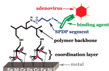
Figure 3. Schematic illustration of adenoviral vector conjugation to a bisphosphonate-modified metal surface for direct gene delivery upon deployment. Reprinted with permission from ref 105. Copyright 2006 National Academy of Sciences, U.S.A.
