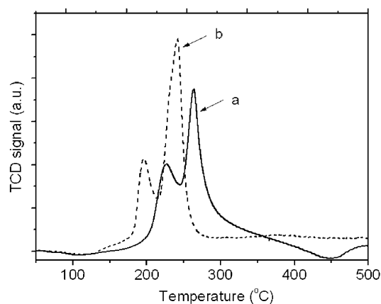
Figure 6. H 2 -TPR profiles of the catalysts: (a) CuO/CeO 2 -nanoparticles and (b) CuO/CeO 2 -nanorods.
