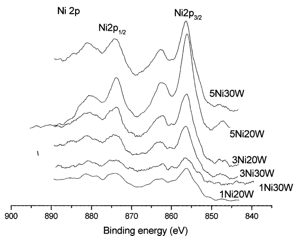
Figure 3. Ni2p photoelectron spectra for NiW / \gamma -Al 2 O 3 catalysts calcined at 400 °C.
