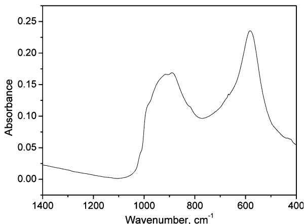
Figure 5. FT-IR spectra of the activated catalyst.
