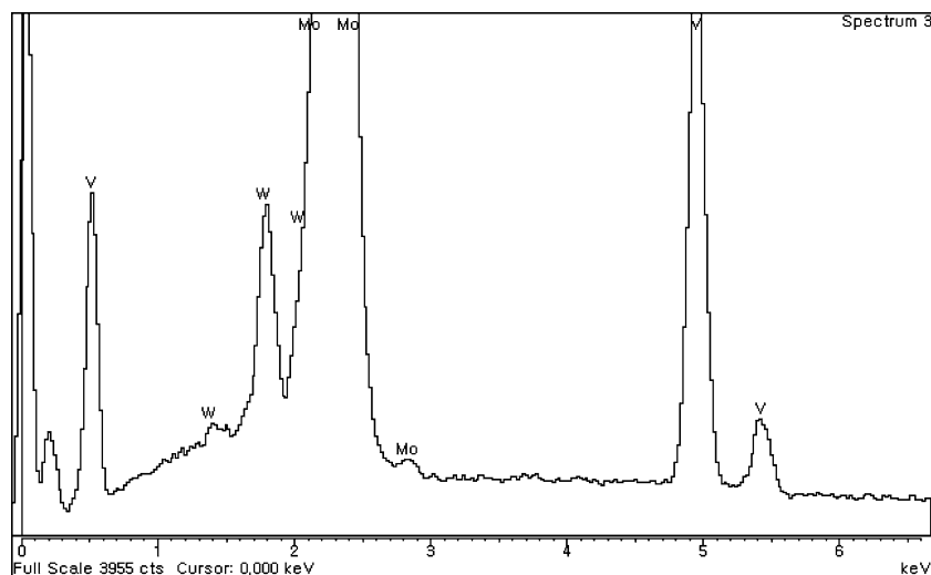
Figure 3. EDX analysis of the activated MoVW catalyst.
