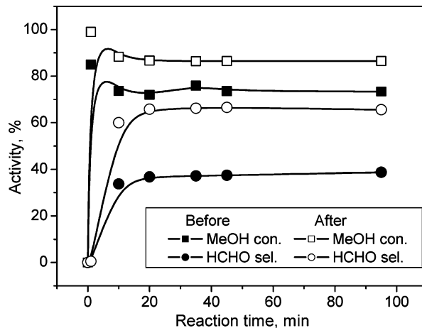
Figure 6. Catalytic activity at 623 K.
