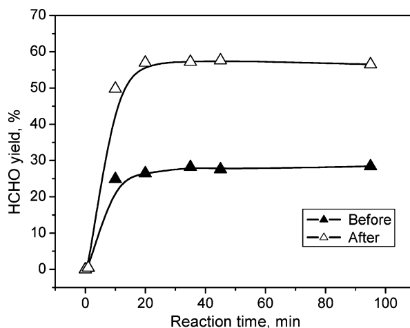
Figure 7. Yield of formaldehyde obtained before and after the thermal treatment of catalyst.
