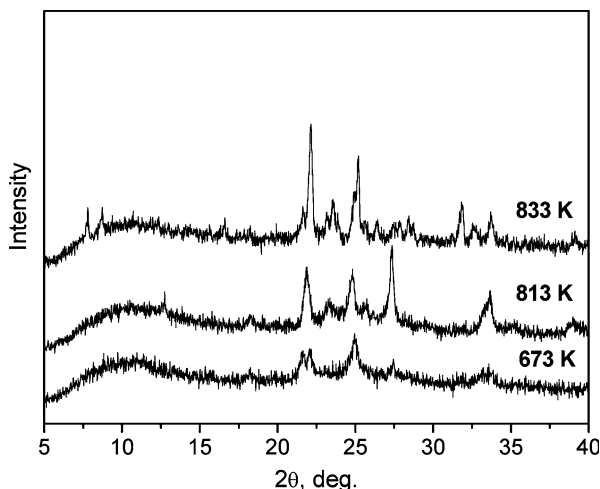
Figure 4. XRD pattern of the catalyst activated at different temperatures.
