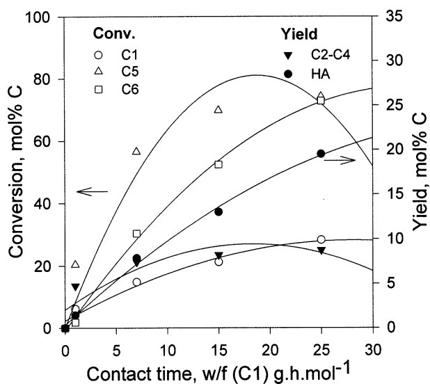
Figure 2. C5, C6, C1 conversion and C2–C4 light hydrocarbons and aromatic hydrocarbons vs. C1 contact time. Temperature: 500 °C. Total pressure: 1 atm. Feed: C1 fraction molar: XC1 = 0.50; TOS = 0, on Zn/H-ZSM-11(c) catalyst.
