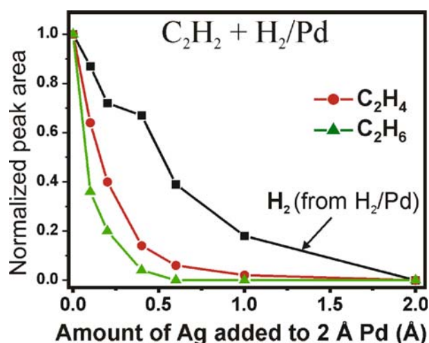
Figure 4. Normalized peak areas of ethane and ethylene produced in co-adsorption experiments (acetylene on H-precovered surface) as a function of amounts of Ag added to Pd. The amounts of hydrogen available in the particles before acetylene adsorption is also shown.
