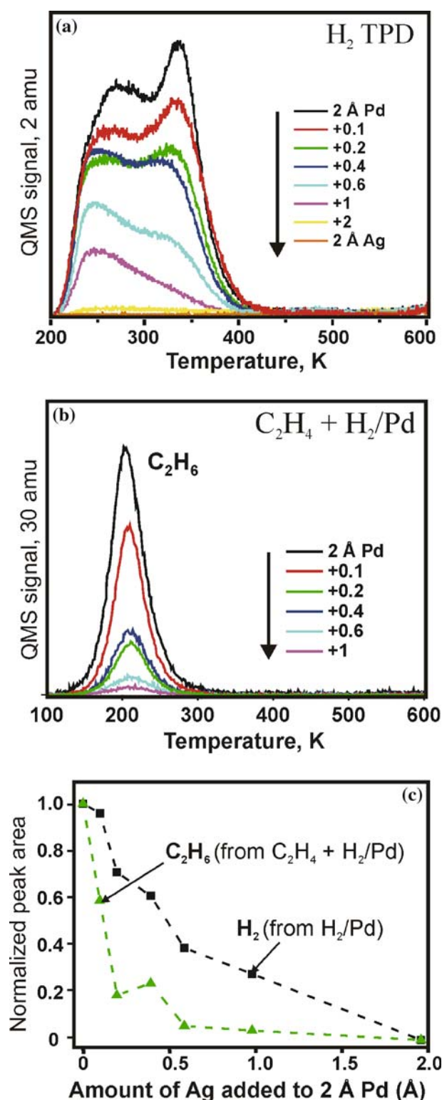
Figure 3. (a) H_2 TPD spectra of Pd-Ag particles for different amounts of Ag added to 2 Å of Pd deposited on alumina film as indicated. The spectra for pure Pd and Ag are also included, for comparison. All samples were exposed to 2 L of H_2 at 200 K. (b) TPD signals of ethane after 1.5 L of ethylene was dosed at 100 K to the surface pre-exposed to 2 L of H_2 at 200 K. (c) Normalized peak areas of ethane produced in co-adsorption experiments and of hydrogen available in the system before ethylene adsorption.
