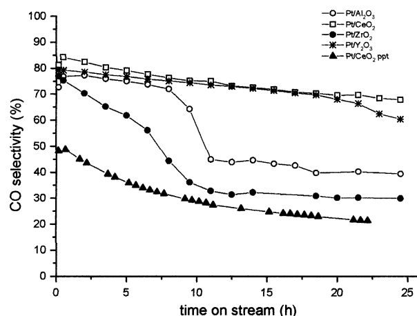
Figure 6. Selectivity to CO in the partial oxidation of methane on Pt Catalysts ( P = 1 atm, T = 800 °C, CH 4 :O 2 = 2:1, WHSV = 523 h -1 ).
