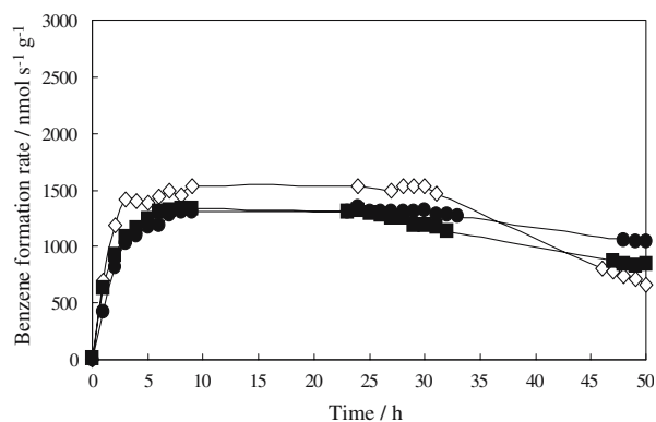
Figure 4. Time course of benzene formation rates over noble metal promoted Mo/HMCM-22 (Rh or Pt/Mo = 0.2). The reaction was performed under conditions of 1023 K, 0.3 MPa and 2700 ml h -1 of CH 4 space velocity with 9% H 2 addition. \diamond : Mo/HMCM-22, \blacksquare : Rh-Mo/HMCM-22, \bullet : Pt-Mo/HMCM-22.
