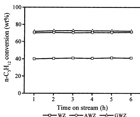
Figure 3. Catalytic activity of WZ, AWZ and GWZ catalysts for n -pentane isomerization as a function of time. P = 2 MPa, T = 215 °C, H_2/n\text{-C}_5 = 3 and WHSV = 1 h -1 .
