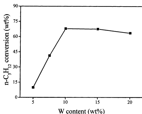
Figure 5. Effect of W content on catalytic performance of AWZ. Data obtained after 6 h on feed. P = 2 \text{ MPa} , T = 215^{\circ}\text{C} , \text{H}_2/n\text{-C}_5 = 3 and \text{WHSV} = 1 \text{ h}^{-1} .
