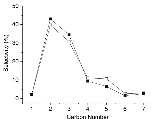
Figure 5. Product distribution in carbon number of chloromethane conversion over SAPO-34 (LS)-□ and SAPO-34 (HS)-■ ( T = 450\text{ }^{\circ}\text{C} , Reaction time = 65 min).
