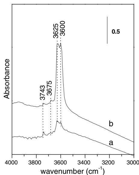
Figure 3. FTIR spectra of activated SAPO-34 (LS)-a and SAPO-34 (HS)-b.
