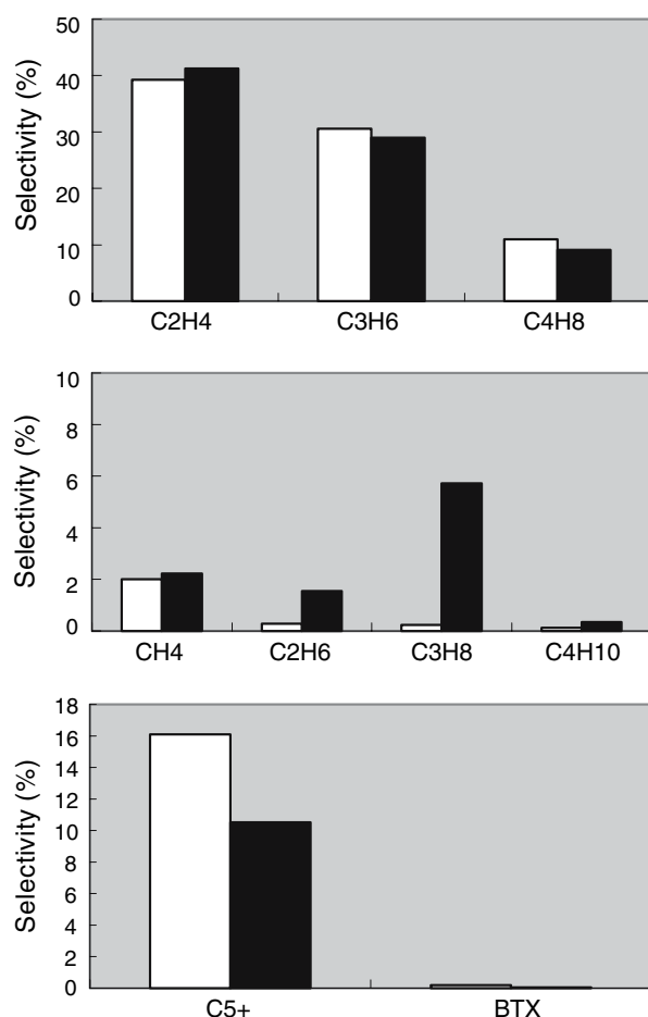
Figure 6. Product selectivity of chloromethane transformation over SAPO-34 (LS)-□ and SAPO-34 (HS)-■ ( T = 450\text{ }^{\circ}\text{C} , Reaction time = 65 min).
