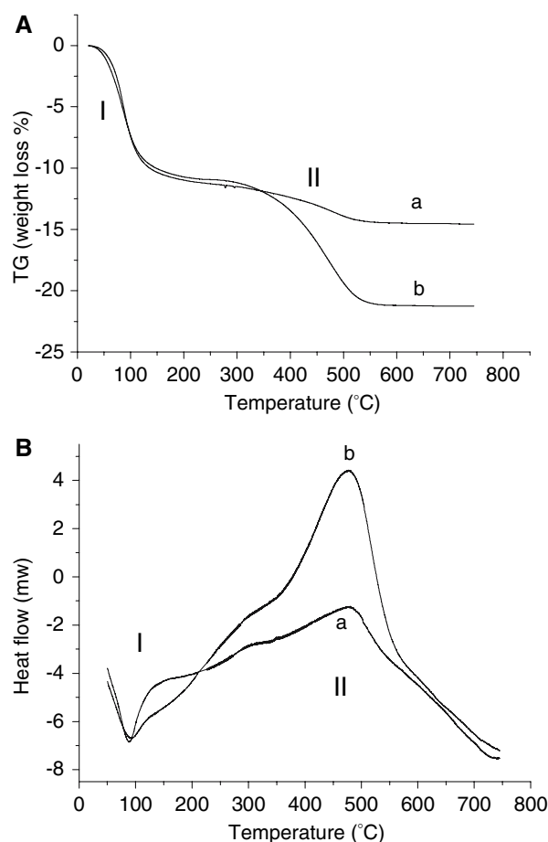
Figure 7. Thermal analysis (TG-A and DSC-B) of discharged catalysts SAPO-34(LS)-a and SAPO-34(HS)-b after reaction at 450 ^{\circ}\text{C} for 65 min.
