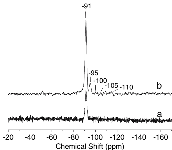
Figure 2. ^{29}\text{Si} MAS NMR spectra of SAPO-34 (LS)-a and SAPO-34 (HS)-b.
