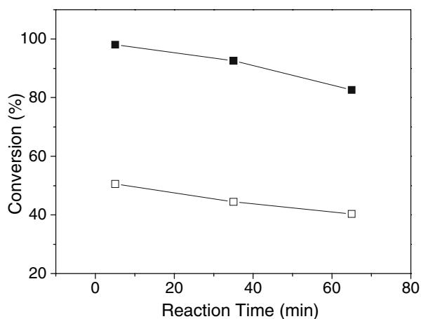
Figure 4. Chloromethane conversion over SAPO-34 (LS)-□ and SAPO-34 (HS)-■ with reaction time ( T = 450\text{ }^{\circ}\text{C} ).
