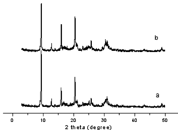
Figure 1. XRD patterns of the as-synthesized samples, (a) SAPO-34(LS) (b) SAPO-34(HS).
