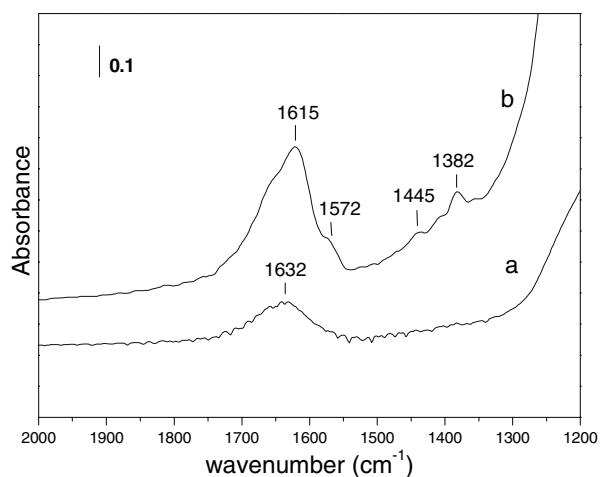
Figure 8. FTIR analysis of discharged catalysts SAPO-34(LS)-a and SAPO-34(HS)-b after reaction at 450 °C for 65 min.
