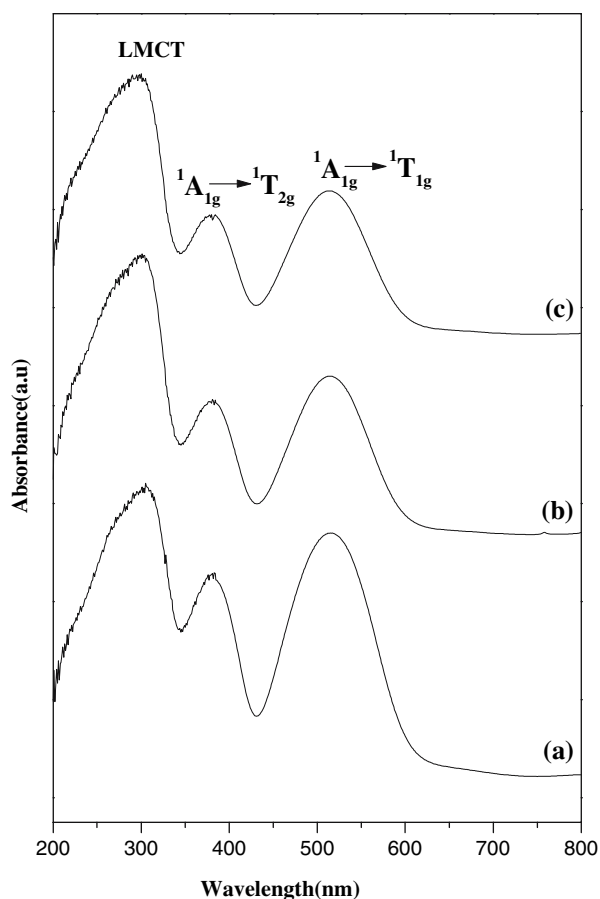
Figure 2. UV-visible spectra of \{M(H_2O)_3Co[C_5N_1H_3(COO)_2]_3\} : (a) M = Gd (1), (b) M = Dy (2) and (c) M = Y (3).
