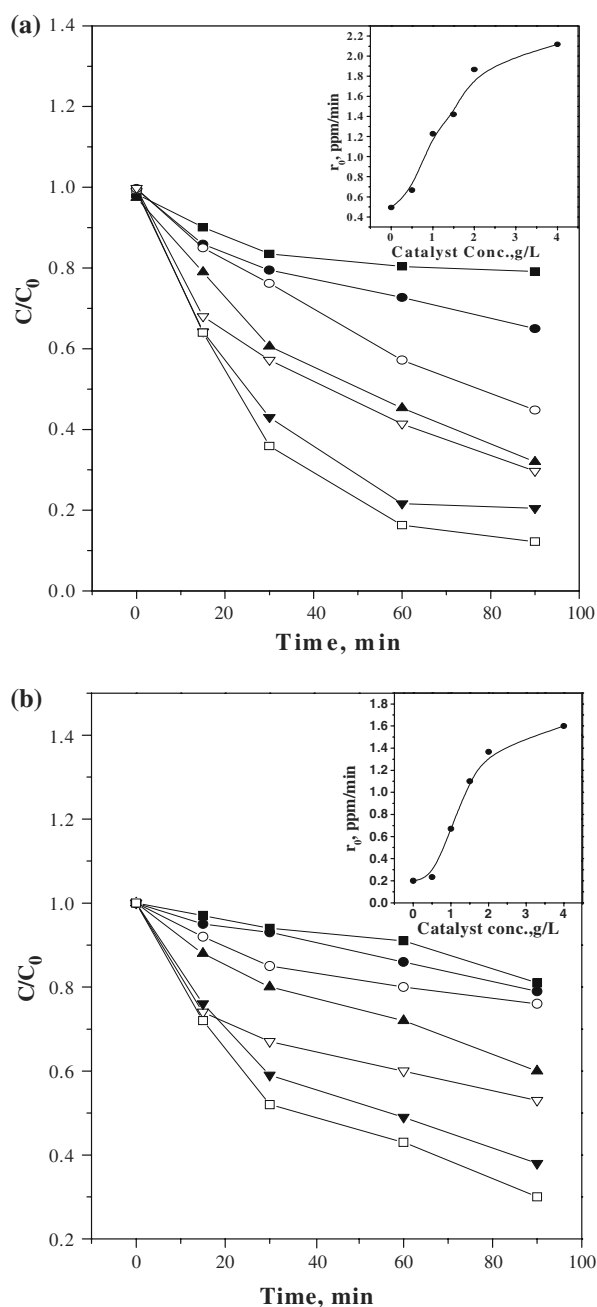
Figure 3. Degradation profiles for 100 ppm RBBR (a) or OG (b) without 1 (■), with 0.5 g/L (●), 1 g/L (▲), 1.5 g/L (▼), 2 g/L (▽), 4 g/L of 1 (□), with 1 g/L of Degussa P-25 (○). Inset shows the variation of the degradation rate with the catalyst concentration.
