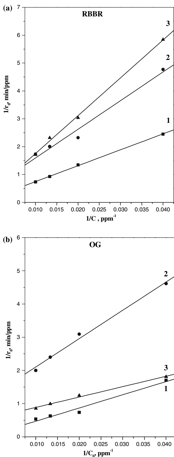
Figure 4. The variation of the initial photodegradation rate with the initial concentration of RBBR (a) and OG (b) by 1, 2 and 3.
