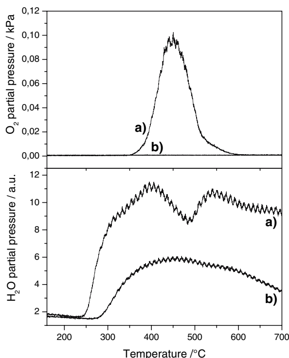
Figure 3. \text{O}_2 -TPD (top panel) and \text{H}_2\text{O} -TPD (bottom panel) of (a) pure ceria and (b) a \text{Au/CeO}_2 catalyst after reductive pre-treatment at 200^\circ\text{C} , recorded in a \text{N}_2 stream ( 12\ \text{N ml min}^{-1} , 5^\circ\text{C min}^{-1} ).
