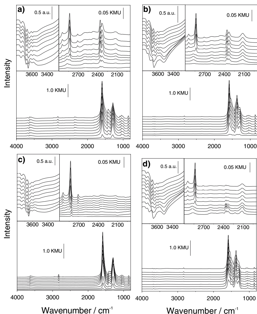
Figure 5. Series of DRIFT spectra obtained during the WGS reaction in idealized reformate (dilute water gas, 0.5 kPa CO, 1 kPa H 2 O, the rest N 2 ) over 1000 min on Au/CeO 2 catalysts pre-treated at 200 °C in (a) 10% H 2 /N 2 and (b) 10% O 2 /N 2 and at 400 °C in (c) 10% H 2 /N 2 and (d) 10% O 2 /N 2 . Bottom: full spectrum, top left: detail spectra of the O–H region (raw data), top right detail spectra of the C–H region; from bottom to top after 23 s, 35 s, 47 s, 2 min, 4 min, 10 min, 30 min, 60 min, 240 min, 1000 min.
