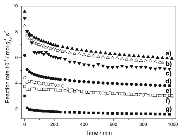
Figure 4. Initial activity and deactivation of differently pre-treated \text{Au/CeO}_2 catalysts in the WGS reaction in idealized reformat ( 1\ \text{kPa CO} , 2\ \text{kPa H}_2\text{O} , rest \text{N}_2 ) at 180^\circ\text{C} . Pre-treatment: (a) 200^\circ\text{C} in 10\%\ \text{H}_2/\text{N}_2 , (b) 200^\circ\text{C} in 10\%\ \text{O}_2/\text{N}_2 , (c) 200^\circ\text{C} in \text{N}_2 , (d) 300^\circ\text{C} in 10\%\ \text{H}_2/\text{N}_2 , (e) 300^\circ\text{C} in 10\%\ \text{O}_2/\text{N}_2 , (f) 400^\circ\text{C} in 10\%\ \text{O}_2/\text{N}_2 and (g) 400^\circ\text{C} in 10\%\ \text{H}_2/\text{N}_2 (other parameters see text).
