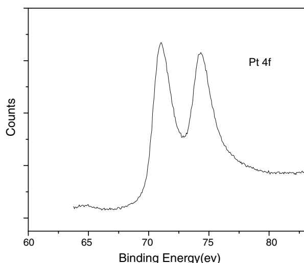
Fig. 3 XPS response of Pt-dendrimer nanocomposite covalently linked to the gold substrate
