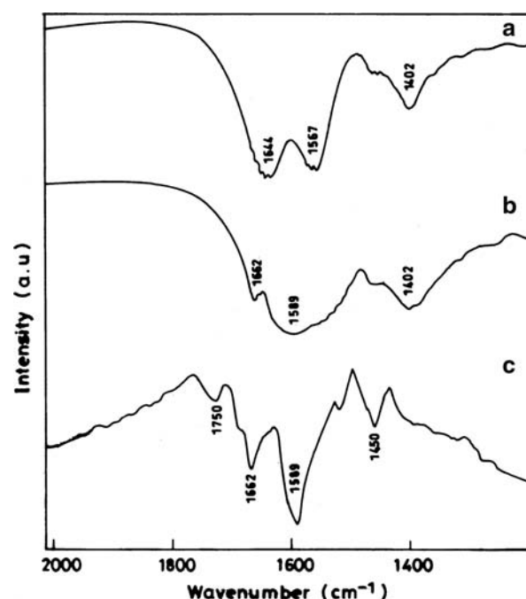
Fig. 4 FTIR spectrum of (a) G-4.5 dendrimer (b) Pt-dendrimer nanocomposite covalently linked to the gold substrate
