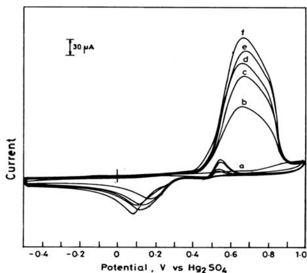
Fig. 7 Cyclic voltammograms representing the methanol oxidation on Pt-dendrimer nanocomposite modified gold substrate for different concentrations of methanol. Scan rate: 50 \text{ mV}/\text{s}^{-1} (a) 0 M; (b) 0.024 M; (c) 0.048 M; (d) 0.072 M; (e) 0.096 M; (f) 0.12 M
