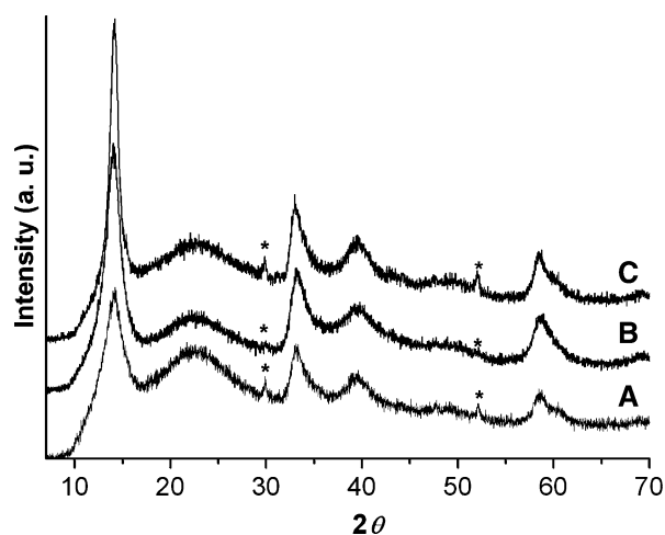
Fig. 2 Wide-angle XRD patterns of (A) \text{Co(2)Mo(10)/SBA-15} (6 nm), (B) \text{Co(2)Mo(20)/SBA-15} (6 nm); (C) \text{Co(3)Mo(14)/SBA-15} (6 nm). (*) \text{Co}_9\text{S}_8
