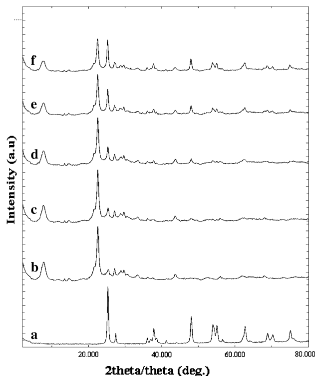
Fig. 3 X-ray diffraction pattern of (a) TiO 2 ; (b) H \beta and (c) 2, (d) 5, (e) 10 and (f) 15 wt.% TiO 2 loaded H \beta zeolite supported systems
