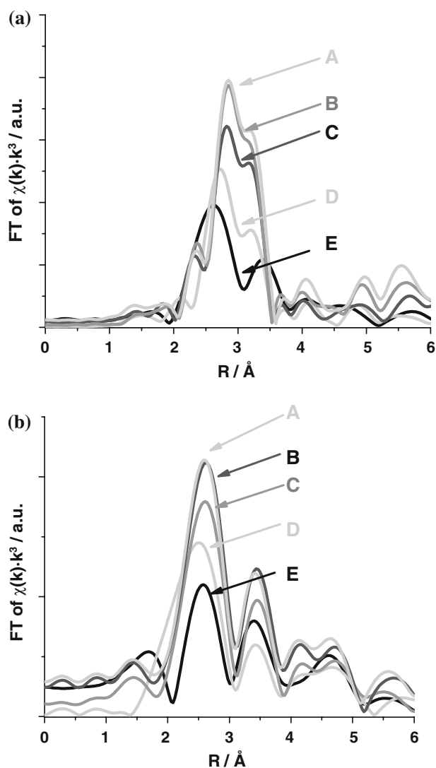
Fig. 3 Fourier transformed EXAFS spectra ( k^3 -weighted \chi(k) function) recorded for the colloids of different size prepared and immobilized on two metal oxide supports: (a) Au on \text{TiO}_2 ; E: 1.3 nm, D: 2.1 nm, C: 6.9 nm, B: 11.3 nm, A: spectrum gold foil for comparison; note that the k -range for E was only 2.5–8 \text{\AA}^{-1} (b) Au on \text{CeO}_2 ; E: 1.3 nm, D: 2.1 nm, C: 6.9 nm B: 11.3 nm, A: gold foil for comparison
