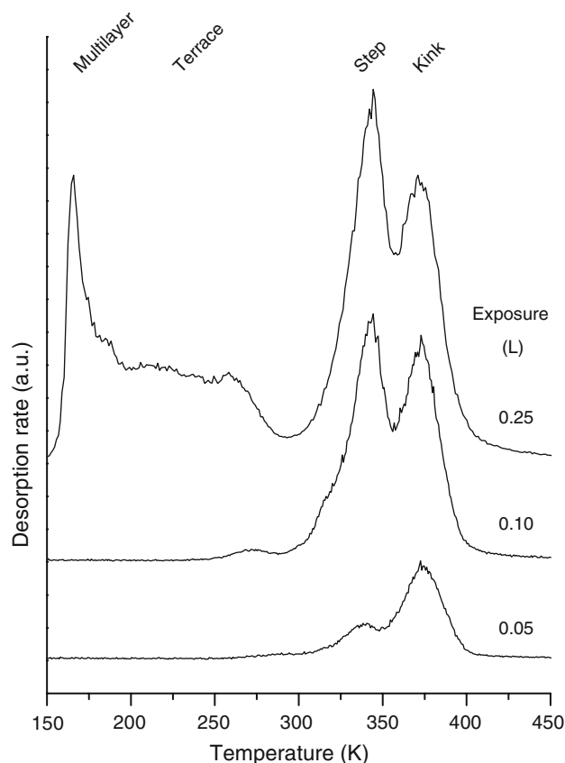
Fig. 2 TPD spectra of ( R )-3-methylcyclohexanone on the \text{Cu}(531)^S surface. The data shown was obtained by monitoring the signal at m/q = 69 using the QMS. The exposure is in units of Langmuir (1 L = 1.0 \times 10^{-6} Torr s). The highest temperature desorption peak at \sim 375 K is assigned to the desorption of ( R )-3-methylcyclohexanone from the kink sites of \text{Cu}(531)^S . The desorption peak at \sim 345 K is assigned to the desorption of ( R )-3-methylcyclohexanone from step sites and the broad feature from 200–270 K is assigned to the desorption of ( R )-3-methylcyclohexanone from terrace sites of \text{Cu}(531)^S . The low temperature peak at \sim 165 K is assigned to desorption of the ( R )-3-methylcyclohexanone multilayer
