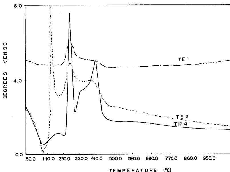
Fig. 2. Differential thermal analysis curves of \text{TiO}_2 synthesized with ethanol (TE1, TE2) and isopropanol (TIP4) as solvents.
