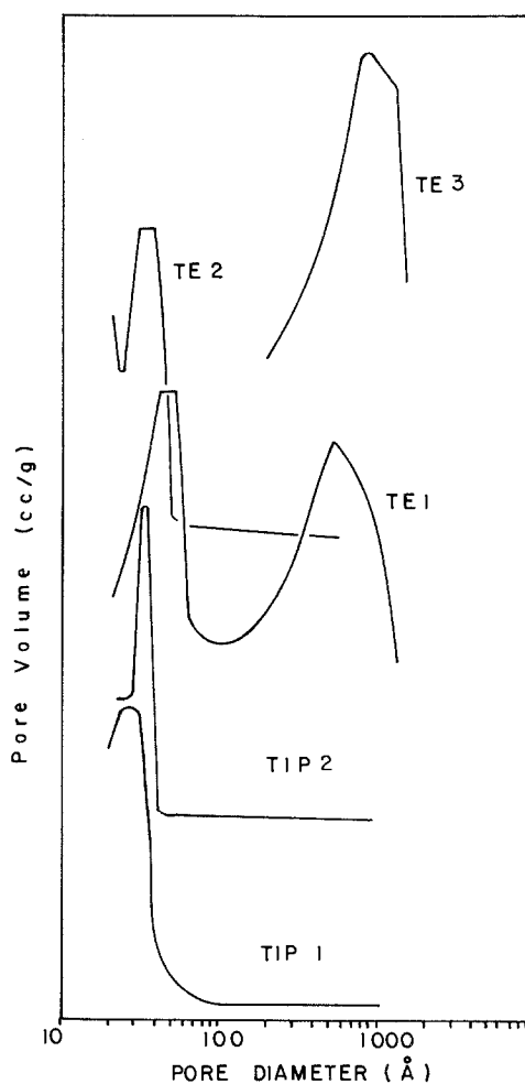
Fig. 5. Pore size distribution of \text{TiO}_2 dried samples (nomenclature as in table 1).
