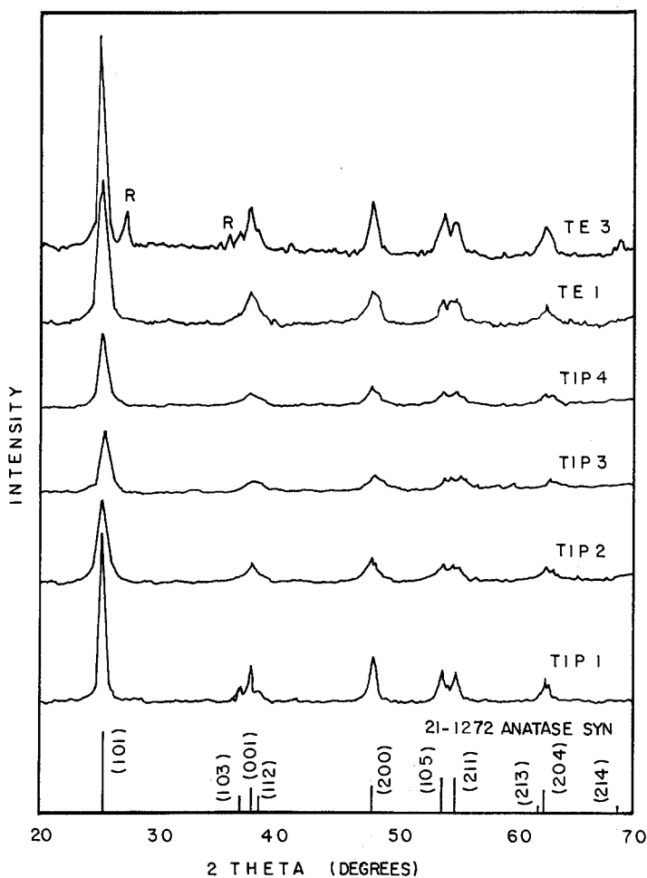
Fig. 4. X-ray diffraction patterns of \text{TiO}_2 calcined samples (R: rutile phase).
