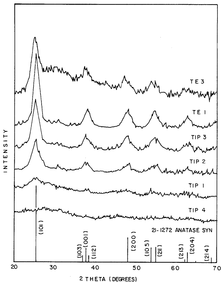
Fig. 3. X-ray diffraction patterns of \text{TiO}_2 dried samples (nomenclature as in table 1).
