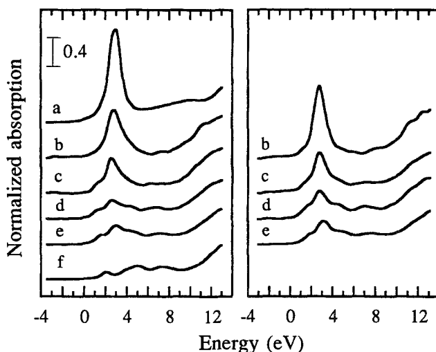
Fig. 5. Pre-edge X-ray absorption spectra (XANES) of samples (a) \text{Ba}_2\text{TiO}_4 , (b) 1TS-48, (c) 2TS-48, (d) 3TS-48, (e) 4TS-48 and (f) anatase before (left) and after (right) dehydration. For the TS-48 samples, the edge position was taken at the maximum of the highest peak.
