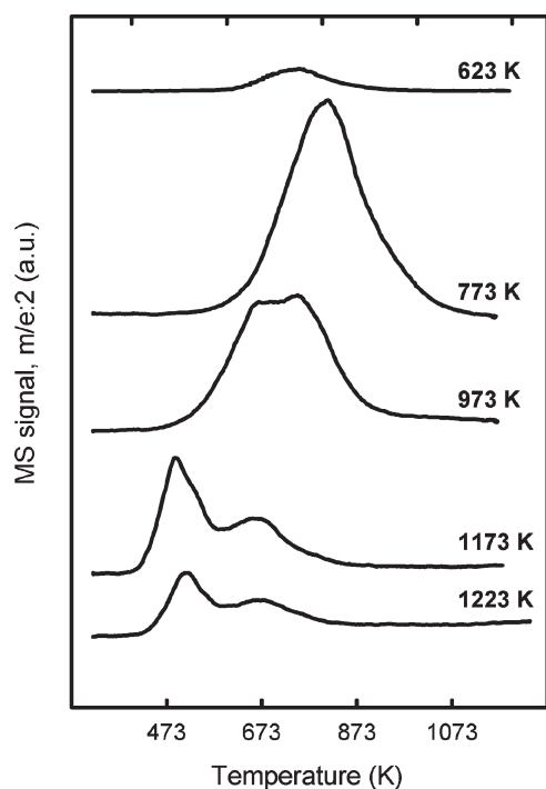
Figure 4. \text{H}_2 -TPD traces of the L40C mixed oxide reduced in a flow of hydrogen for 1 h at the indicated temperatures and cooled down in hydrogen atmosphere.
