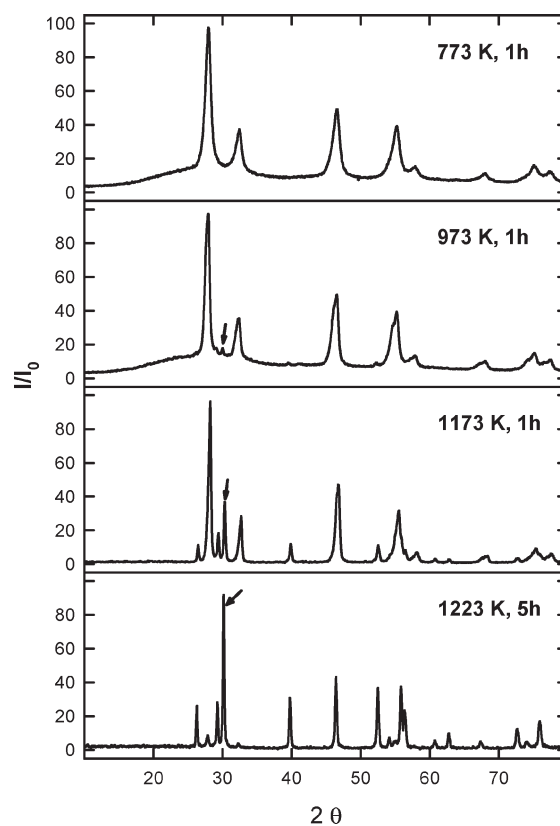
Figure 7. XRD patterns of the L40C mixed oxide after the indicated reduction treatments.
