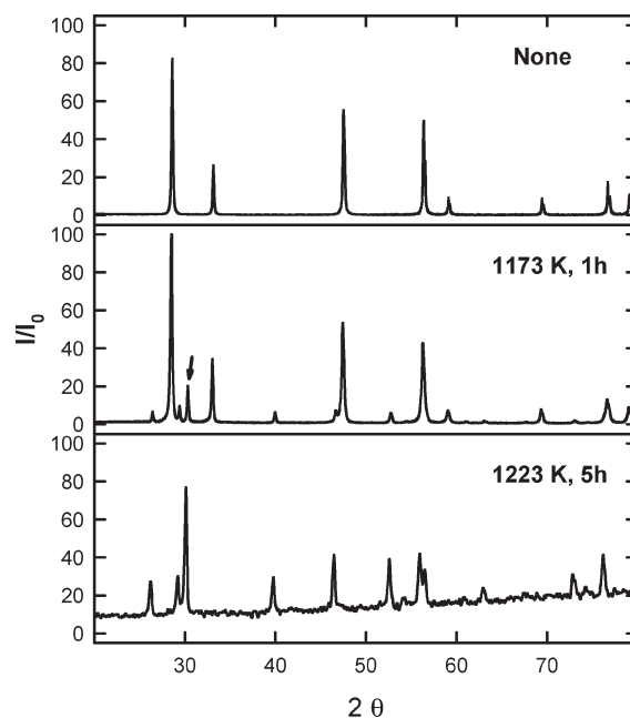
Figure 6. XRD patterns of \text{CeO}_2 after the indicated reduction treatments.
