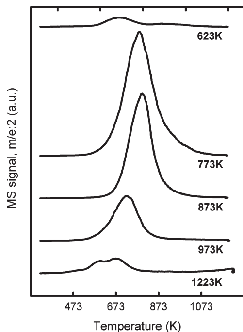
Figure 5. \text{H}_2 -TPD traces of the Y20C mixed oxide reduced in a flow of hydrogen for 1 h at the indicated temperatures and cooled down in a hydrogen atmosphere.
