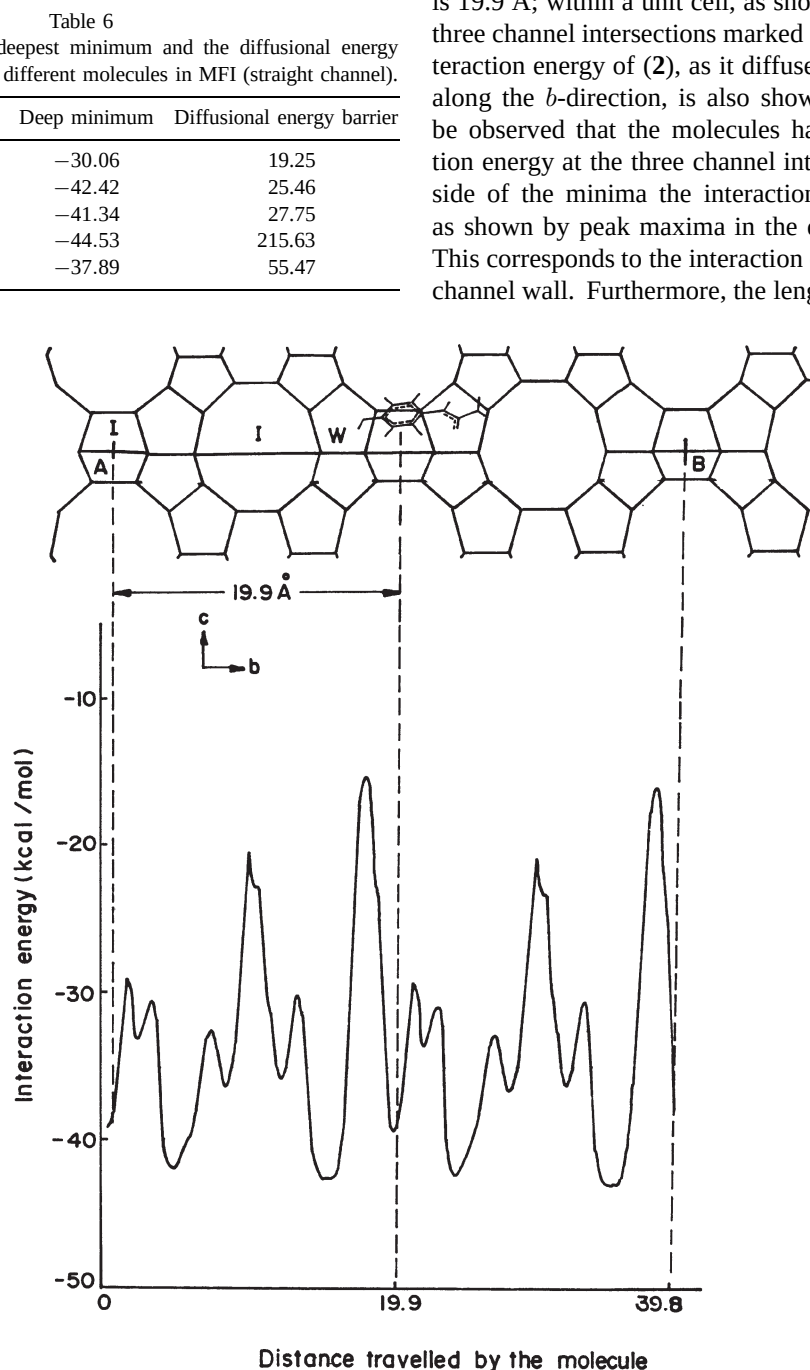
Figure 5. The molecular graphics picture of the cross-sectional view of the 10-MR channel in MFI. The initial and final points (A and B) of the diffusion path are also indicated. A unit cell in b -direction (19.9 Å) has regions of channel intersections (I) and channel walls (W). Variation of interaction energy between the molecule (2) and the MFI framework as the molecule diffuses through the 12-MR channel; the interaction energy variation is symmetrically repeated in every unit cell. A typical configuration for the molecule at a minimum energy location is shown.
