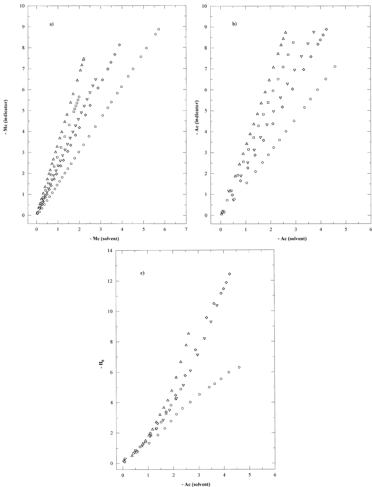
Figure 1. (a) Plot of Mc(\text{indicator}) vs. Mc(\text{solvent}) in: ( \Delta ) MeSO 3 H, ( \square ) HBr, ( \nabla ) HClO 4 , ( \diamond ) CF 3 SO 3 H, ( \circ ) HNO 3 . Mc(i) and Mc(s) values from [6]. (b) Plot of Ac(\text{indicator}) vs. Ac(\text{solvent}) (range > 1 M) in: ( \Delta ) MeSO 3 H ( n_{is} = 3.30 ), ( \square ) HBr ( n_{is} = 2.80 ), ( \nabla ) HClO 4 ( n_{is} = 2.35 ), ( \diamond ) CF 3 SO 3 H ( n_{is} = 2.10 ), ( \circ ) HNO 3 ( n_{is} = 1.55 ). Ac(\text{indicator}) = -n_{is} \log[H^+] + Mc(i) (see equation (15)); Ac(i) , Ac(s) , [H^+] , Mc(i) values from [6]. (c) Plot of H_0 vs. Ac(\text{solvent}) (range > 1 M) in: ( \Delta ) MeSO 3 H, ( \square ) HBr, ( \nabla ) HClO 4 , ( \diamond ) CF 3 SO 3 H, ( \circ ) HNO 3 . Ac(s) values from [6]; H_0 values from [6,10,11] and references therein.
