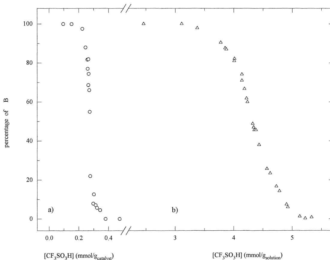
Figure 2. Protonation equilibrium of 2,4-dichloro-6-nitroaniline (B) by UV spectroscopy at 420 nm in: (a) solid phase: percentage of B vs. \text{CF}_3\text{SO}_3\text{H}/\text{SiO}_2 (mmol/g catalyst ); (b) aqueous solution: percentage of B vs. \text{CF}_3\text{SO}_3\text{H} (mmol/g solution ).
