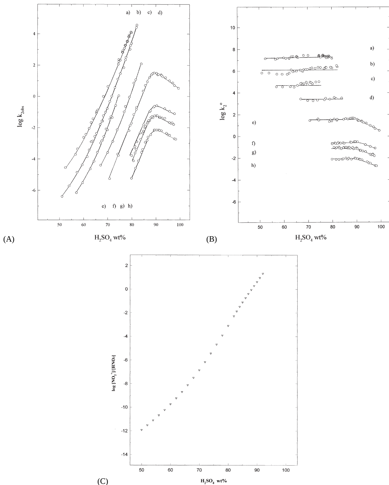
Figure 1. (A) Nitration in aqueous sulfuric acid at 25 °C. Values of \log k_{2\text{obs}} vs. wt% \text{H}_2\text{SO}_4 . (a) Toluene, (b) benzene, (c) bromobenzene, (d) p,p' -dibromobenzene, (e) p -nitrotoluene, (f) o -Cl-nitrobenzene, (g) nitrobenzene, (h) p -Cl-nitrobenzene (experimental data of: (a) from [23–26], (b) from [23,27,28], (c) from [27–29], (d) from [29], (e) from [31], (f) from [31], (g) from [32], (h) from [31]). (B) Nitration in aqueous sulfuric acid at 25 °C. Values \log k_2^0 vs. wt% \text{H}_2\text{SO}_4 . (a) Toluene, (b) benzene, (c) bromobenzene, (d) p,p' -dibromobenzene, (e) p -nitrotoluene, (f) o -Cl-nitrobenzene, (g) nitrobenzene, (h) p -Cl-nitrobenzene (experimental data as in figure 1(A)). (C) Protonation-dehydration equilibrium of nitric acid in aqueous sulfuric acid. Values of \log [\text{NO}_2^+]/[\text{HNO}_3] at 25 °C: range 50–82 wt% \text{H}_2\text{SO}_4 , estimated values; range 85–92 wt% \text{H}_2\text{SO}_4 , experimental data from [21].
