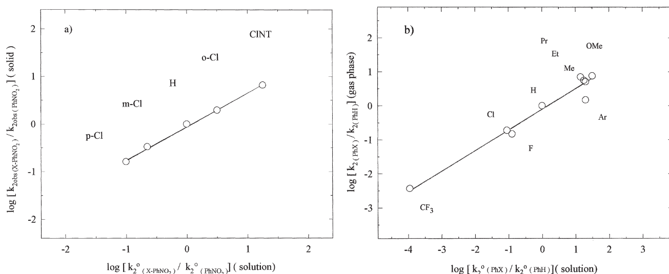
Figure 3. (a) Values of \log[k_{2\text{obs}}(\text{X-PhNO}_2)/k_{2\text{obs}}(\text{PhNO}_2)] (solid-phase nitration) vs. \log[k_{2\text{o}}(\text{X-PhNO}_2)/k_{2\text{o}}(\text{PhNO}_2)] (nitration in aqueous \text{H}_2\text{SO}_4 ) of nitrocompounds: p -chloronitrobenzene ( p -CLNB); m -chloronitrobenzene ( m -CLNB); nitrobenzene (NB); o -chloronitrobenzene ( o -CLNB); p -chloro- m -nitrotoluene (CLNT) (experimental data in solid phase – present work; in liquid phase, ( m -CLNB) and (CLNT) – present work, ( p -CLNB) from [31], (NB) from [32]). (b) Values of \log[k_{2(\text{PhX})}/k_{2(\text{PhH})}] (gas-phase nitration) vs. \log[k_{2\text{o}}(\text{PhX})/k_{2\text{o}}(\text{PhH})] (nitration in aqueous \text{H}_2\text{SO}_4 ) of monosubstituted arenes: anisole (OMe); toluene (Me); ethylbenzene (Et); propylbenzene (Pr); biphenyl (Ar); benzene (H); fluorobenzene (F); chlorobenzene (Cl); benzotrifluoride (CF 3 ) (experimental data in gas phase from [39]; in \text{H}_2\text{SO}_4 from [7]).
