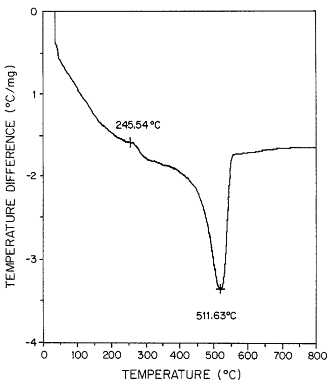
Figure 8. DTA curve of the coked Pt-Sn/ \gamma -Al 2 O 3 catalyst.
