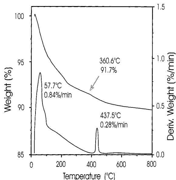
Figure 11. DTG-TG profiles of the regenerated Pt-Sn/ \gamma -Al 2 O 3 catalyst.
