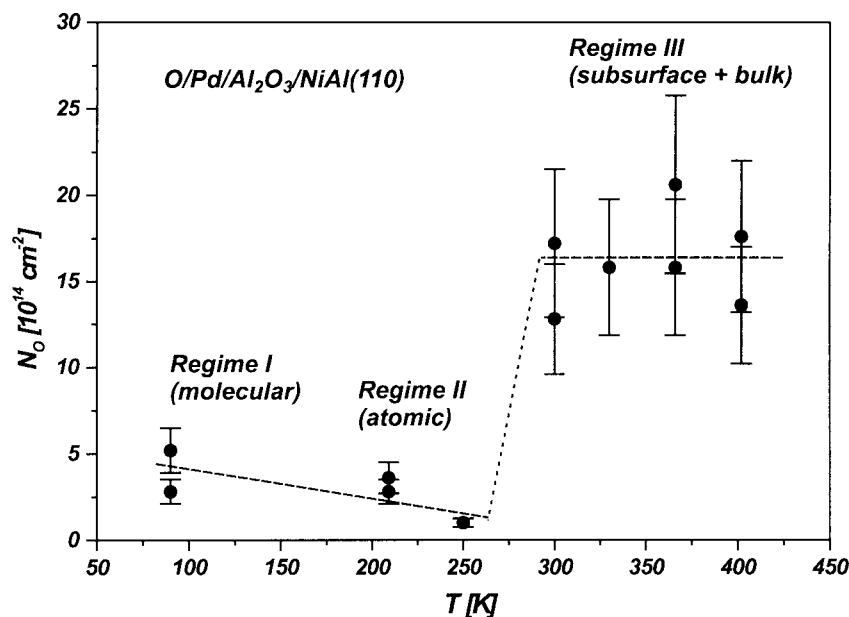
Figure 4. Oxygen uptake (in O-atoms \text{cm}^{-2} ) of a sample of Pd particles supported on \text{Al}_2\text{O}_3/\text{NiAl}(110) directly after preparation under UHV conditions as a function of the sample temperature.
