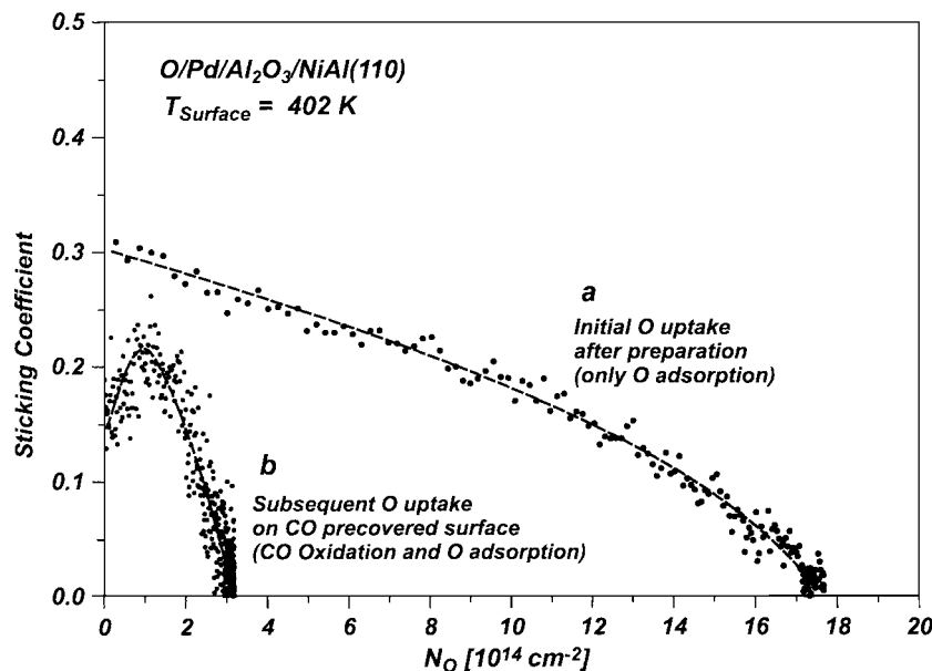
Figure 3. O_2 sticking coefficient as a function of oxygen uptake (in O-atoms cm^{-2} ) at 402 K for Pd particles supported on Al_2O_3/NiAl(110) directly after preparation under UHV conditions and after several cycles of O_2 and CO exposure.
