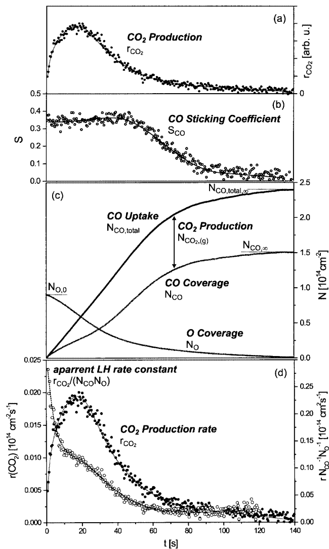
Figure 5. (a) Relative \text{CO}_2 production for O-precovered Pd/ \text{Al}_2\text{O}_3 /NiAl(110) at a sample temperature of 402 K (preparation conditions 1, CO beam 8.6 \times 10^{12} \text{ molecules cm}^{-2} \text{ s}^{-1} ), (b) CO sticking coefficient as a function of experiment time; (c) O and CO surface coverages (see text); (d) absolute \text{CO}_2 production rate and apparent Langmuir–Hinshelwood rate constant.
