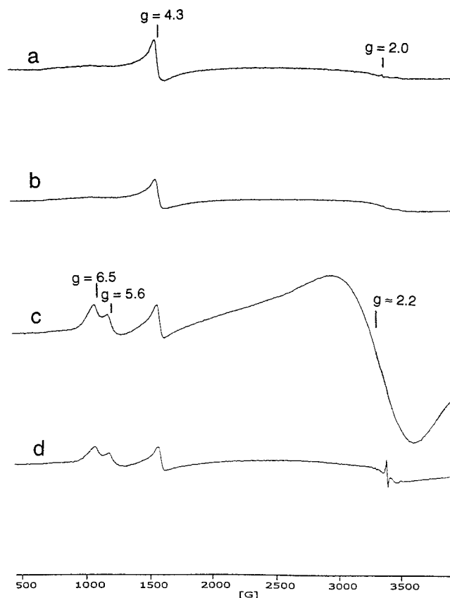
Figure 1. ESR spectra at 20 °C of fresh catalysts: (a) Fe-ZSM-5 (CA: conventional aqueous ion-exchange), (b) Fe-ZSM-5 (IA: improved aqueous ion-exchange), (c) Fe-ZSM-5 (SS: solid-state ion-exchange) and (d) Fe-ZSM-5 (CV: chemical vapor ion-exchange). Detailed preparation conditions of the catalysts are given in table 1.
