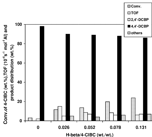
Figure 1. Influence of H-beta/4-ClBC (wt./wt) ratio on the 4-ClBC conversion, TOF and product distribution. Reaction conditions: see the footnotes to table 2.
