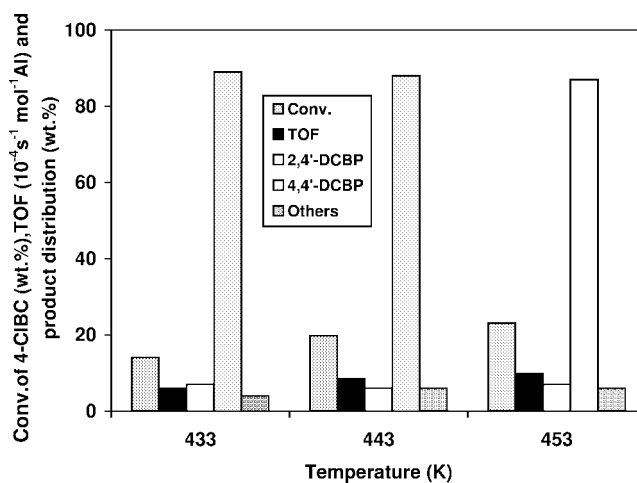
Figure 2. Influence of reaction temperature on the conversion of 4-ClBC, TOF and product distribution. Reaction conditions: see the footnotes to table 2.
