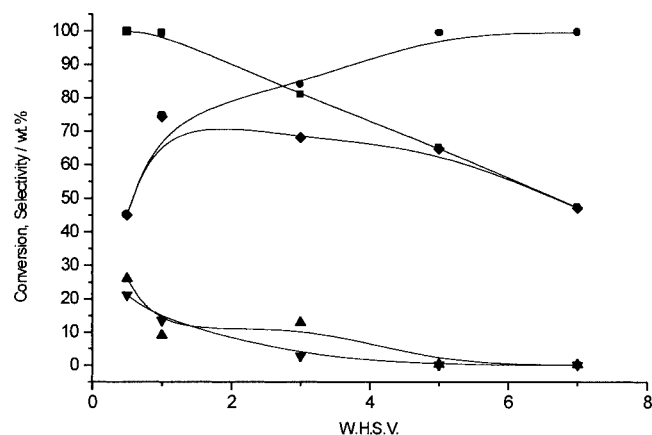
Figure 3. Influence of WHSV data on the conversion and selectivity for Beckmann rearrangement of cyclohexanone oxime over H-ferrierite (■) conversion (wt%) of oxime; (●) selectivity (wt%) of caprolactam, (▲) selectivity (wt%) of cyclohexanone, (▼) selectivity (wt%) of 5-cyano-pent-1-ene and (◆) yield (wt%) of caprolactam. Reaction conditions: temperature = 400 °C, pressure = 1 atm, oxime concentration in feed = 10 wt% in solvent, nitrogen flow rate = 20 ml min -1 , time on stream of the reaction = 3 h, catalyst weight = 3 g.
