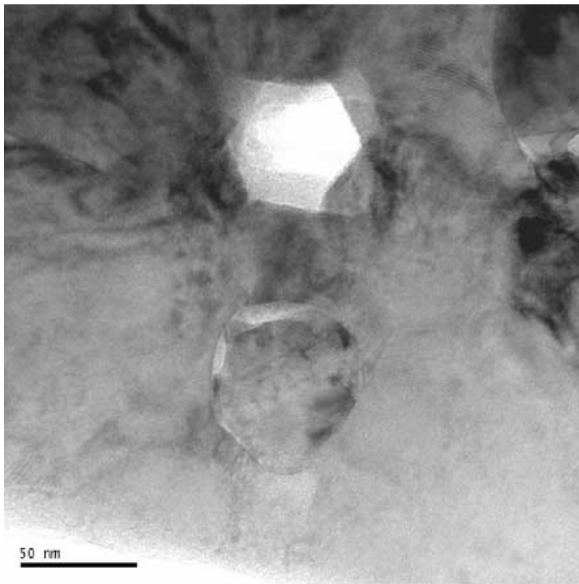
Figure 4. TEM of Pd/ZrO 2 showing encapsulated Pd particles (upper right corner and bottom center) and a void (top center) within the ceria-zirconia matrix.
