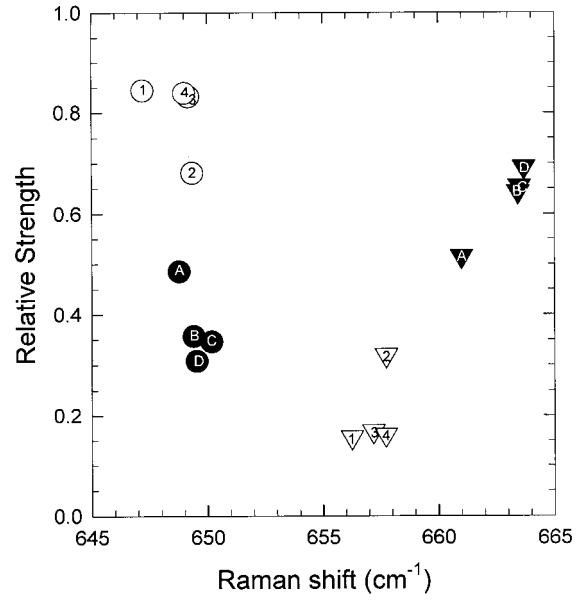
Figure 7. Results of fitting spectra in figure 6 to two Lorentzian lines as explained in the text. Open (filled) symbols represent the light (dark) spheres.
